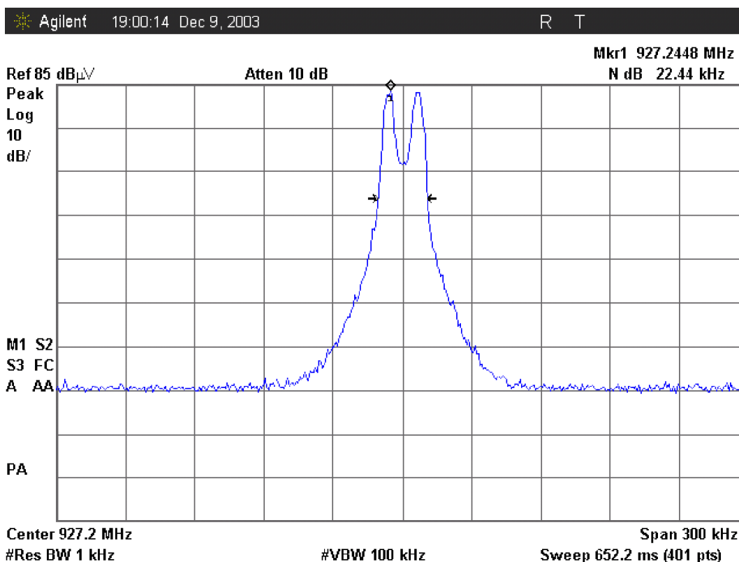
Figure 2: Plot of the Occupied bandwidth (HANDSET, Operating at 927.25 MHz)
