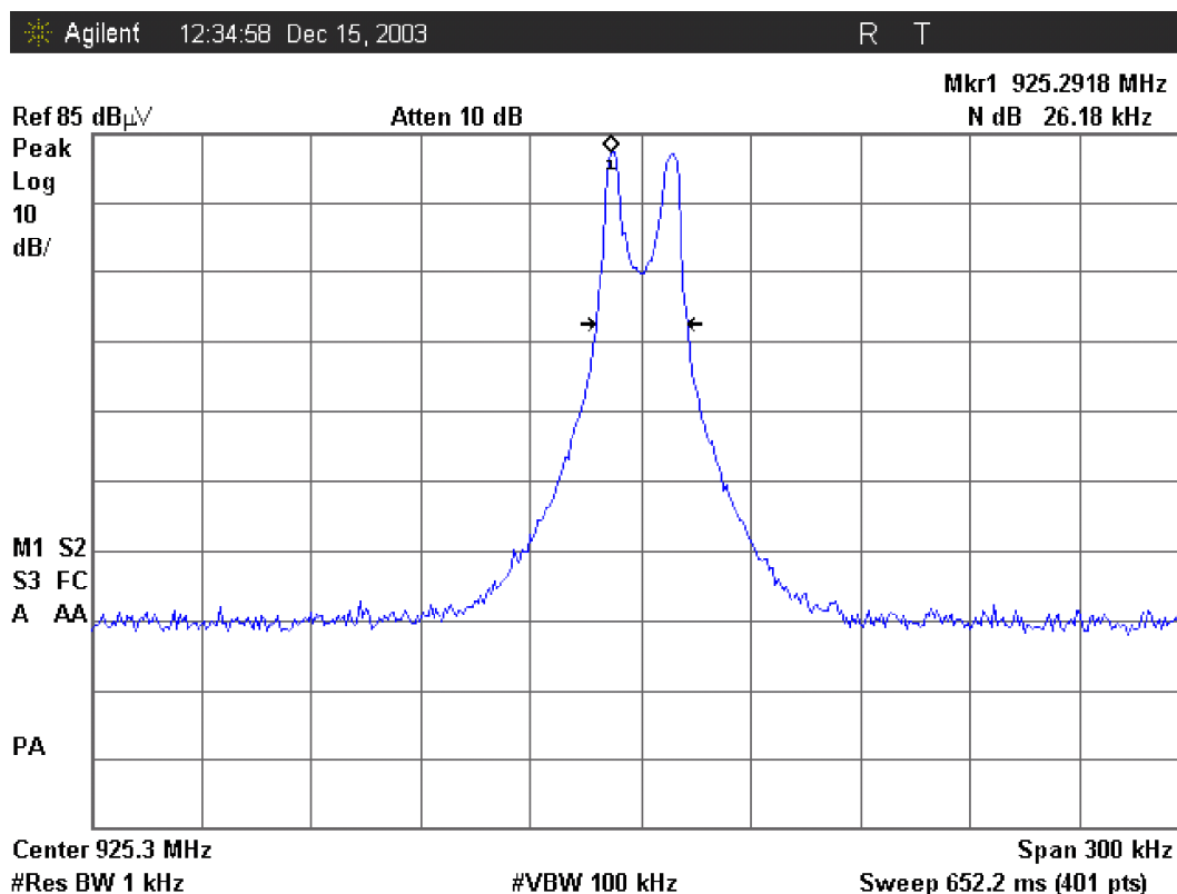
Figure 1: Plot of the Occupied bandwidth (HANDSET, Operating at 925.30 MHz)
