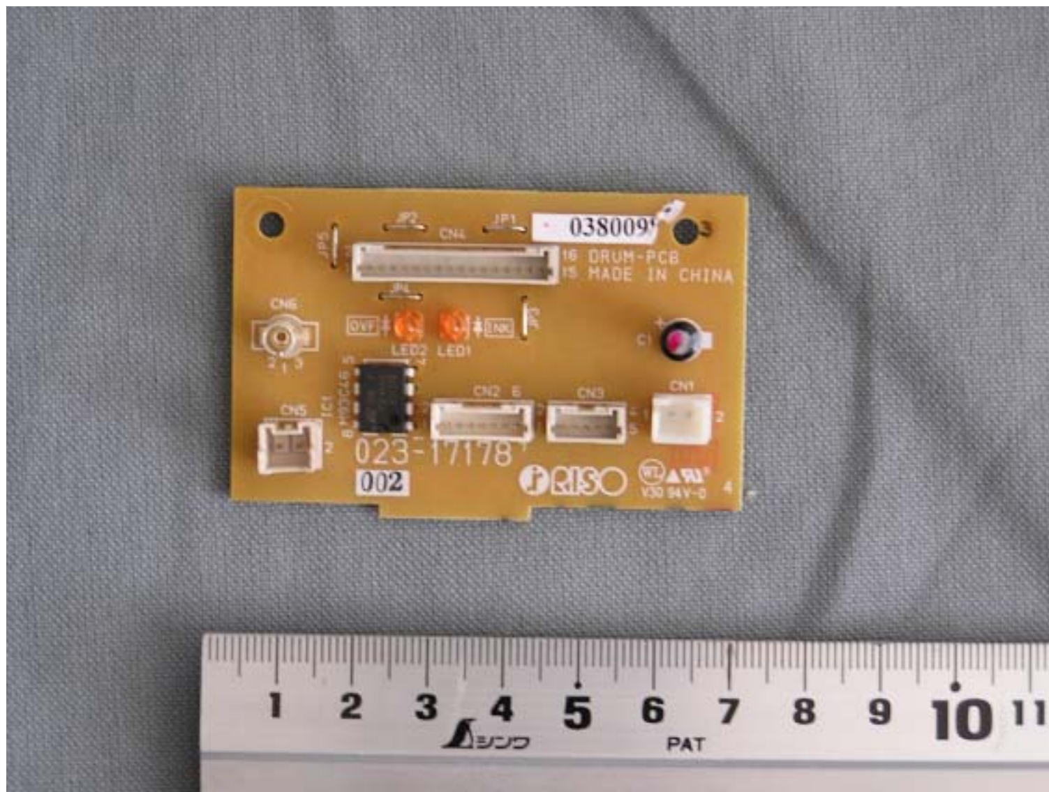
RZ390UI DRUM-PCB Top View
