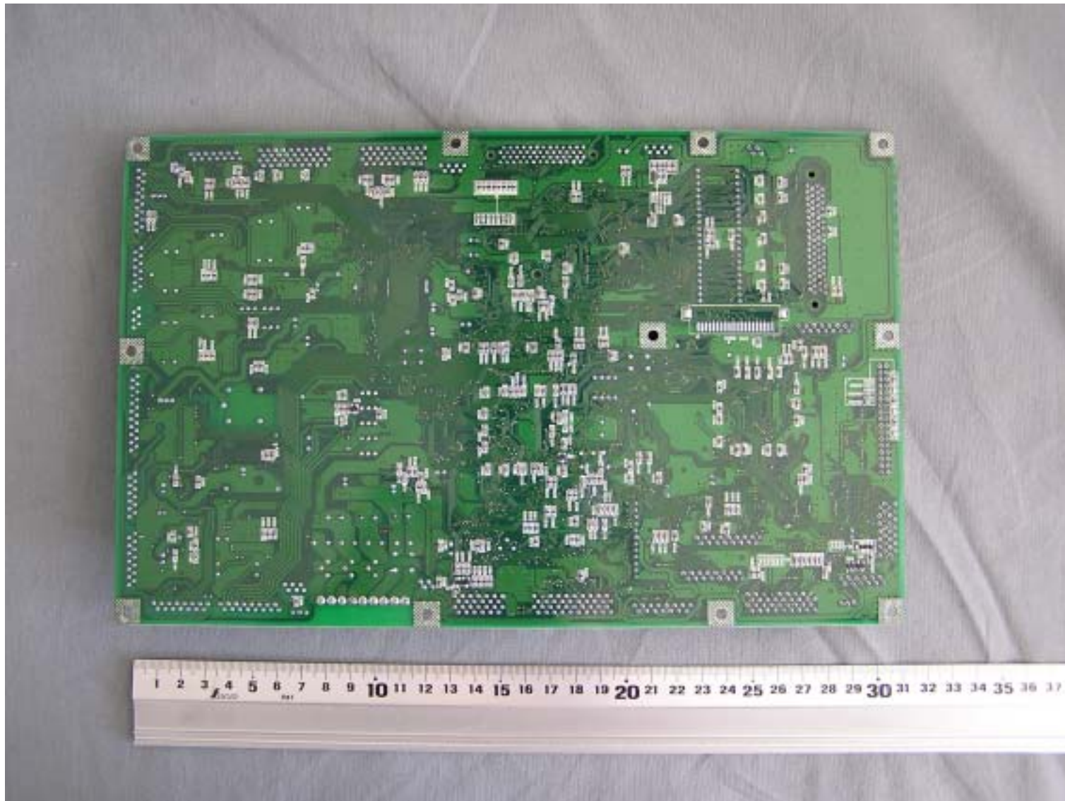
RZ390UI DuplicatorCTL-PCB Bottom View
