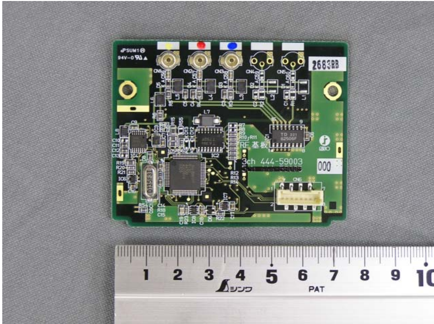
RZ390UI RF-Module Top View
