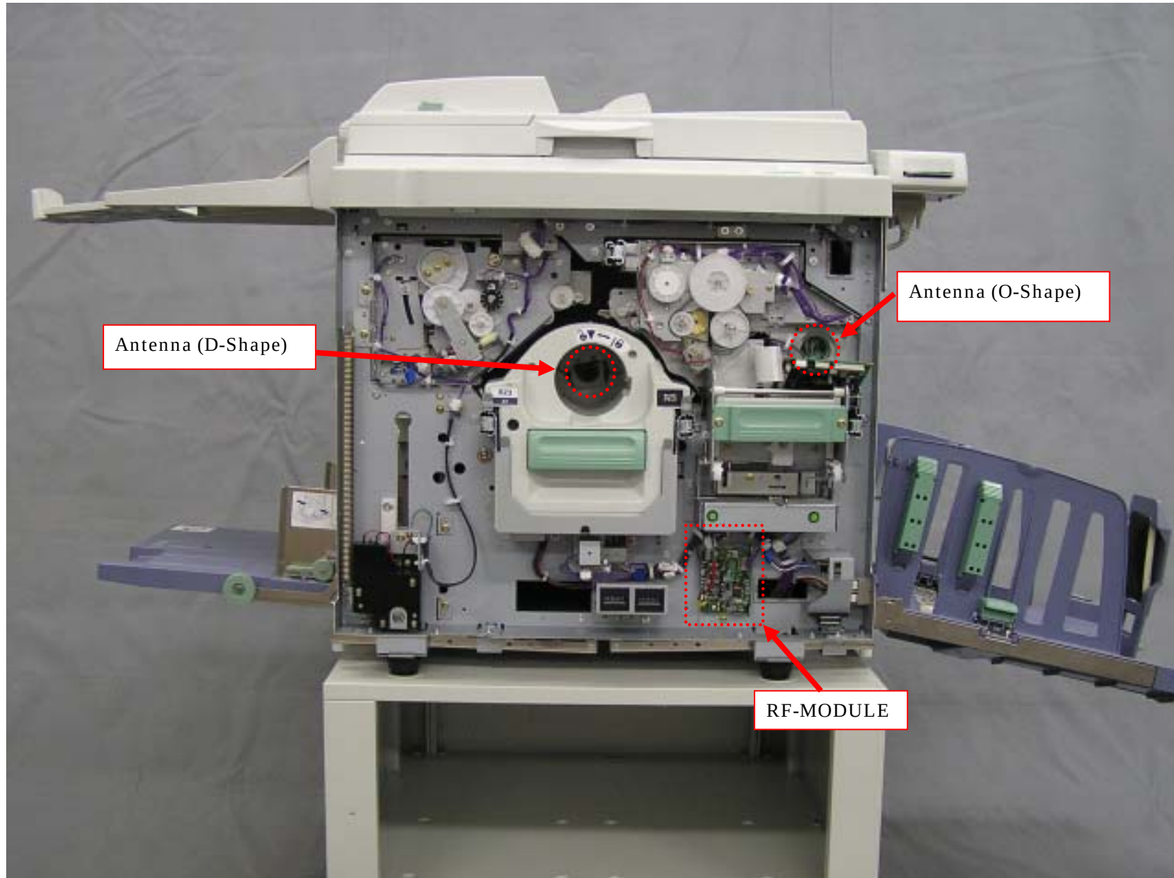
RZ390UI Duplicator Front View Cover Open
