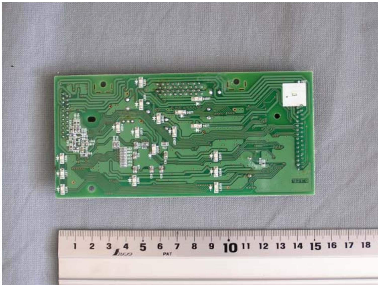
RZ390UI Operation Panel Bottom View
