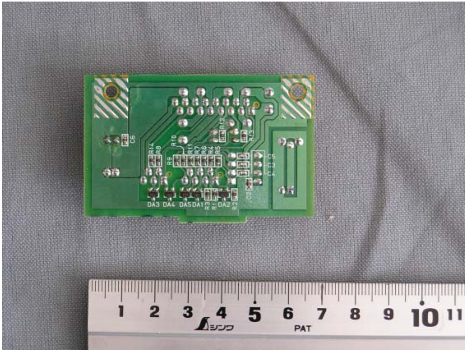
RZ390UI DRUM-PCB Bottom View
