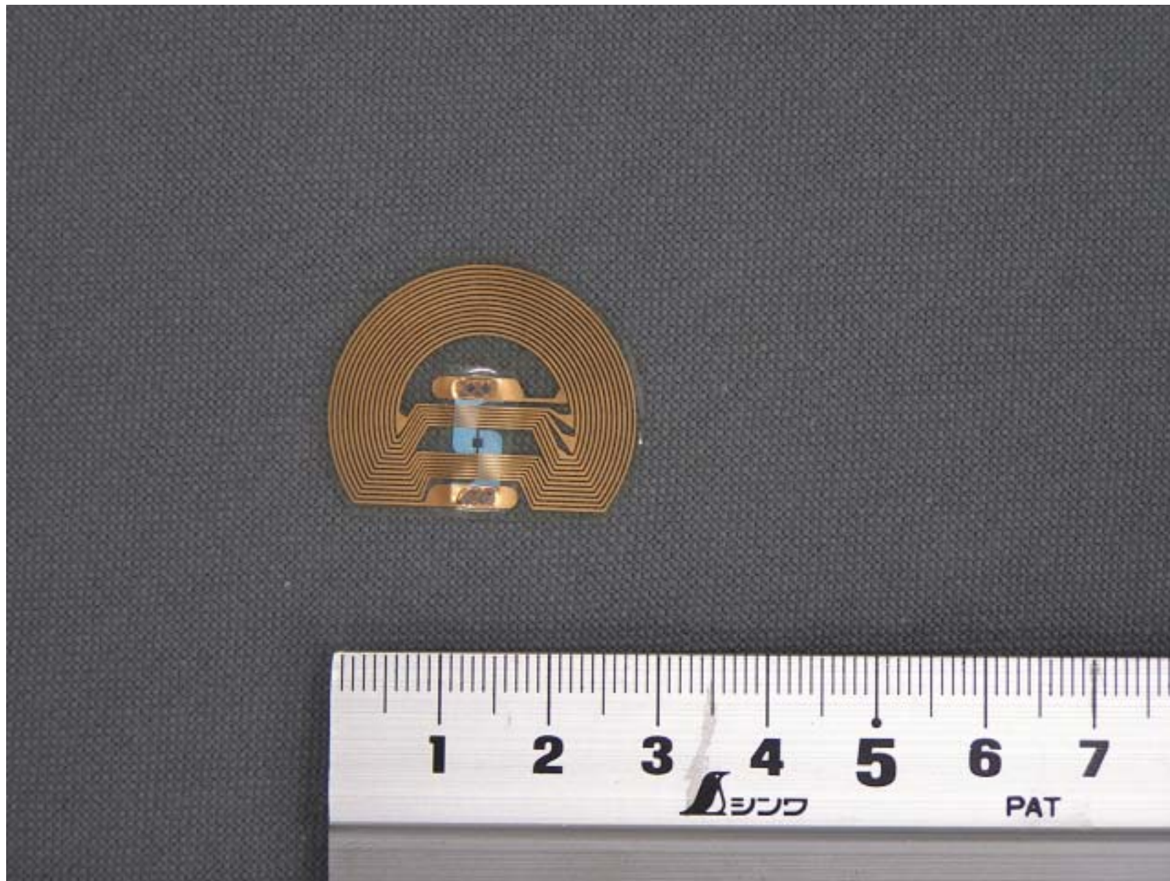
RZ390UI RF-Tag Top View
