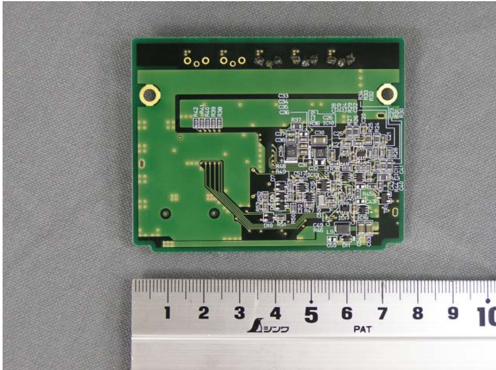
RZ390UI RF-Module Bottom View
