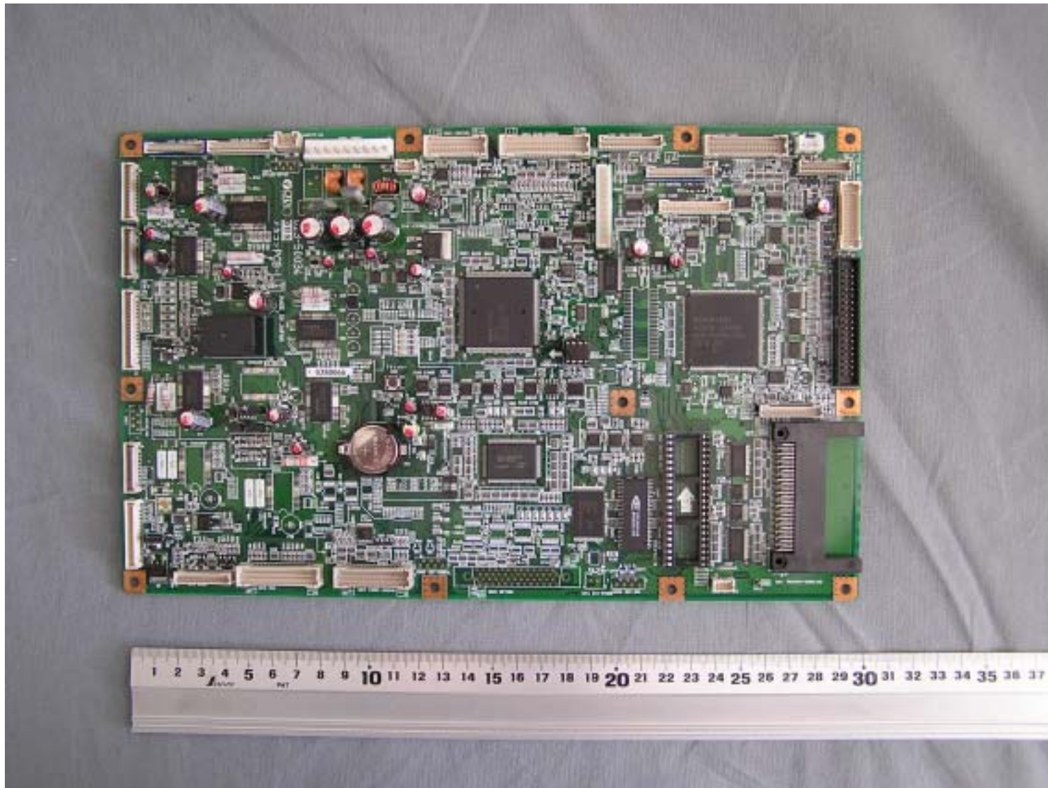
RZ390UI Duplicator CTL-PCB Top View
