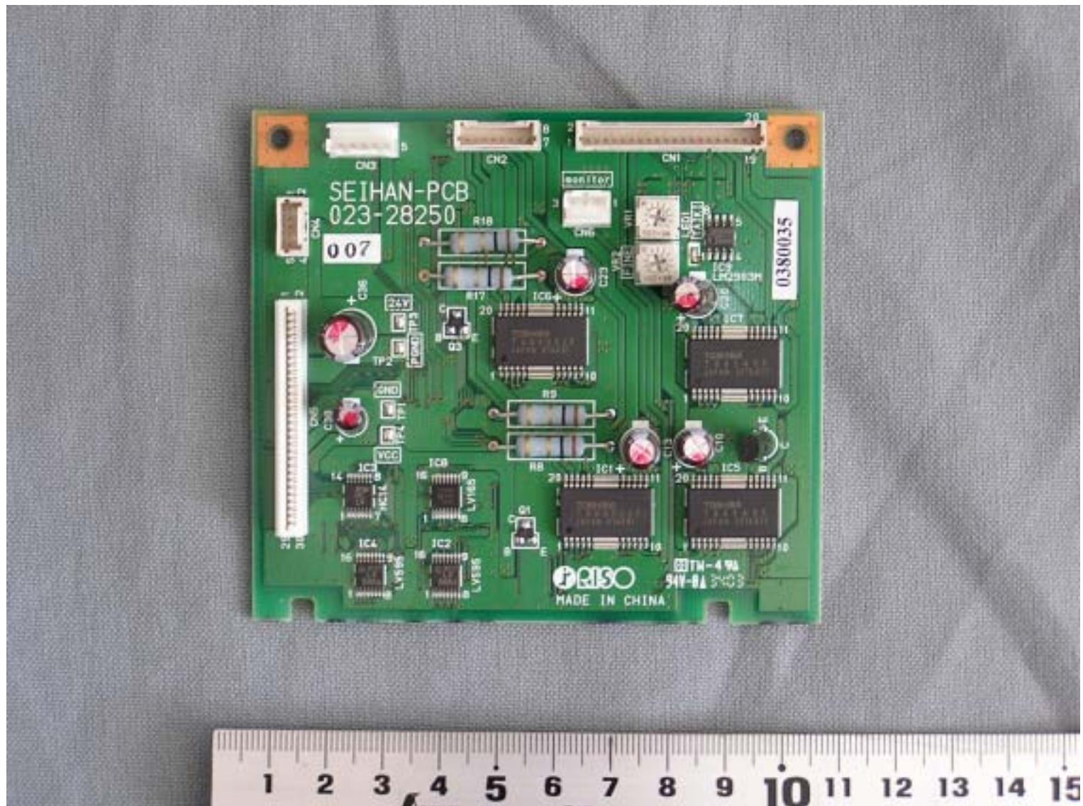
RZ390UI Master Making-PCB Top View
