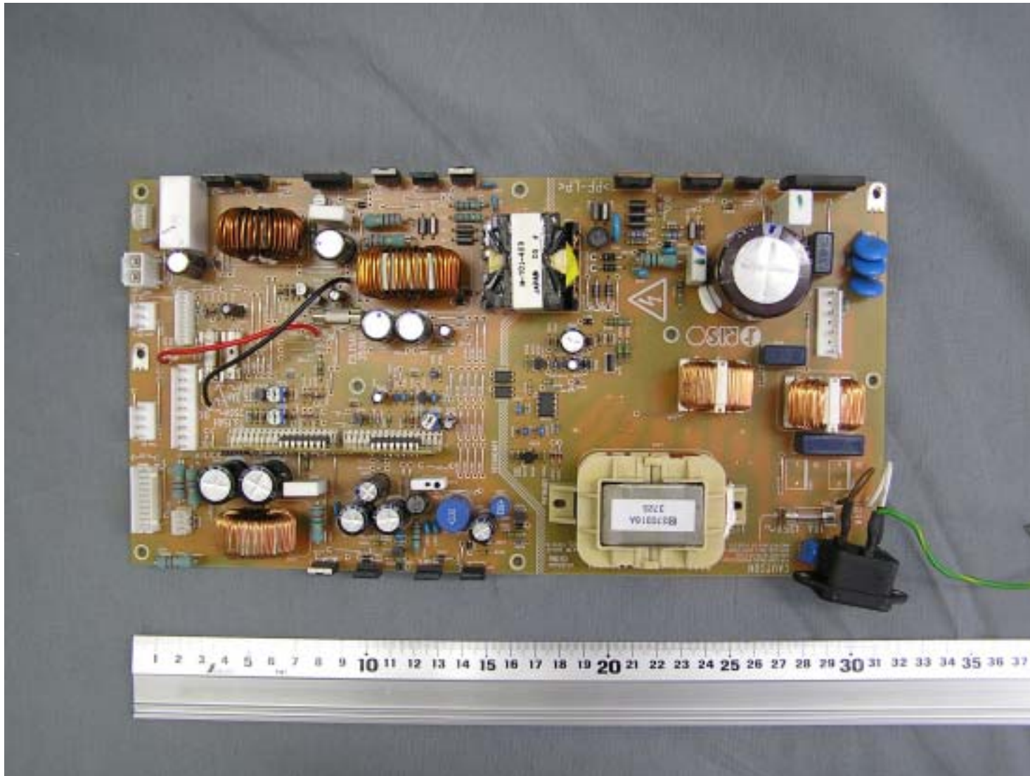
RZ390UI Power Supply Top View
