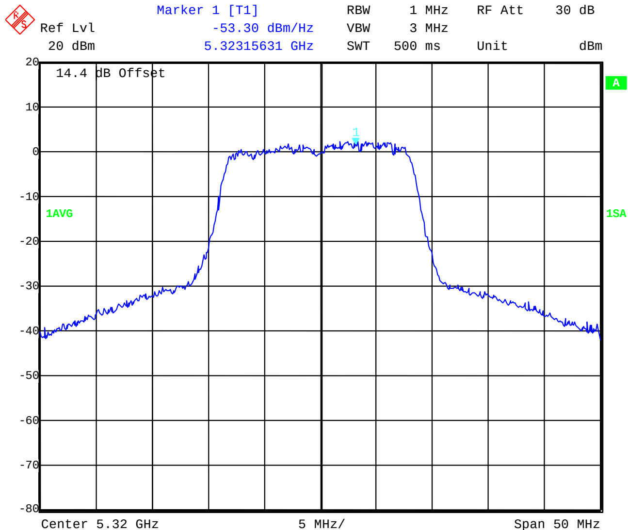
Plot 2: 5320 MHz
