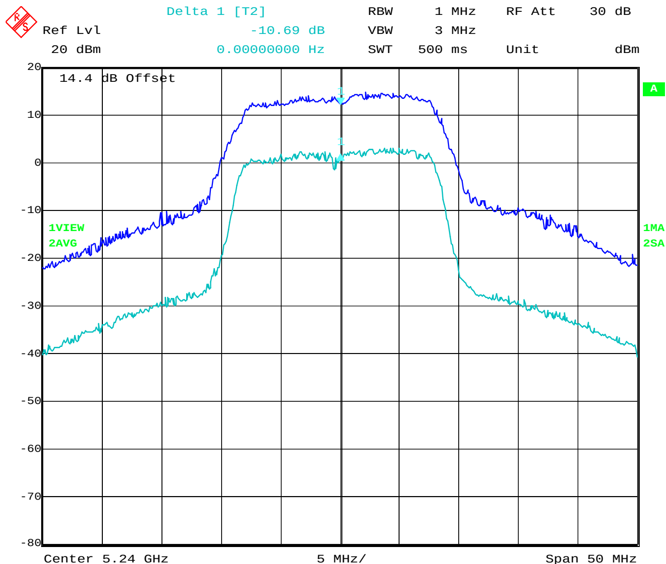
Plot 2: 5240 MHz
