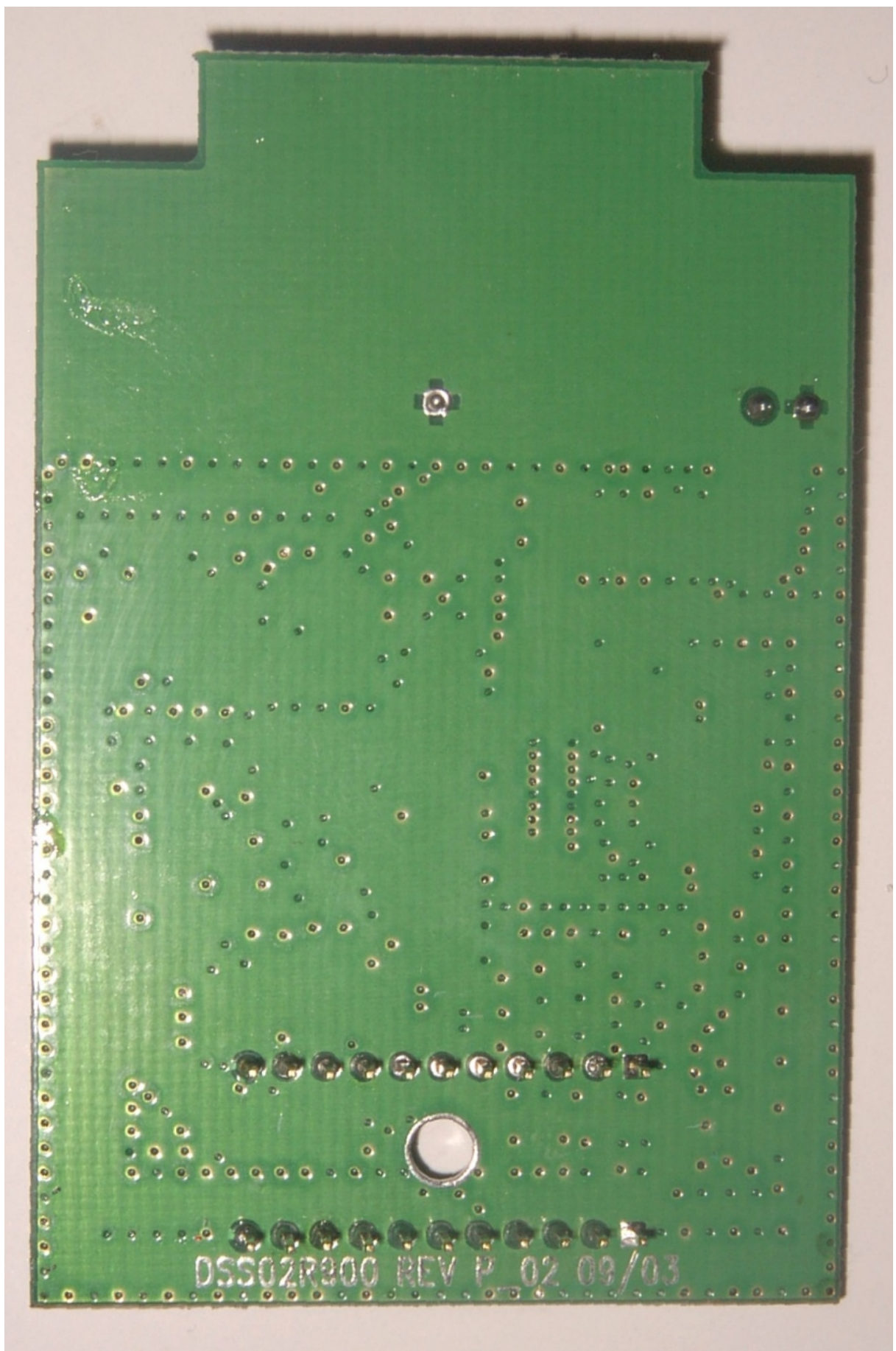
HANDSET RADIO PCB SOLDER SIDE
