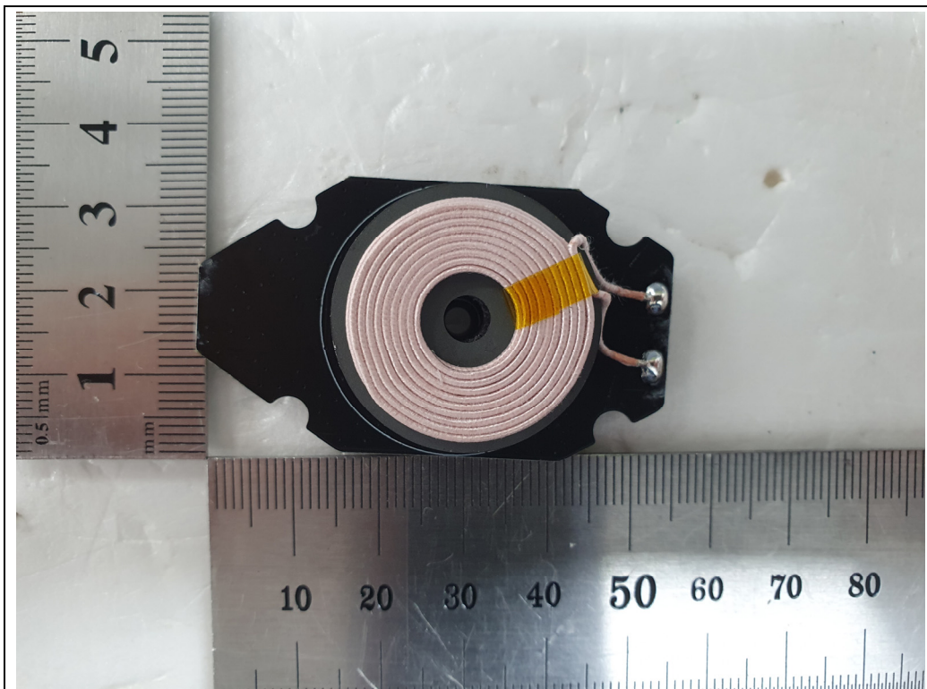
<Coil Antenna>
