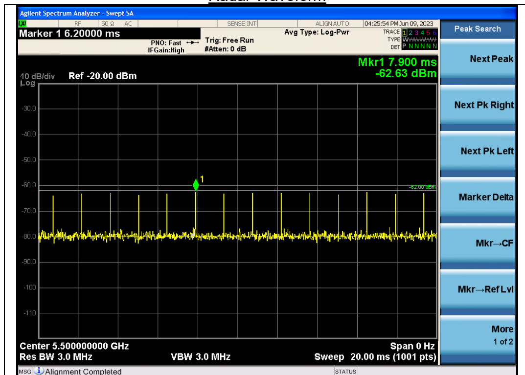
Radar Waveform
