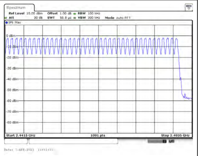
2441.5 ~ 2483.5 MHz
