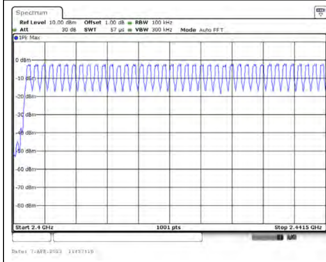
2400 ~ 2441.5 MHz
