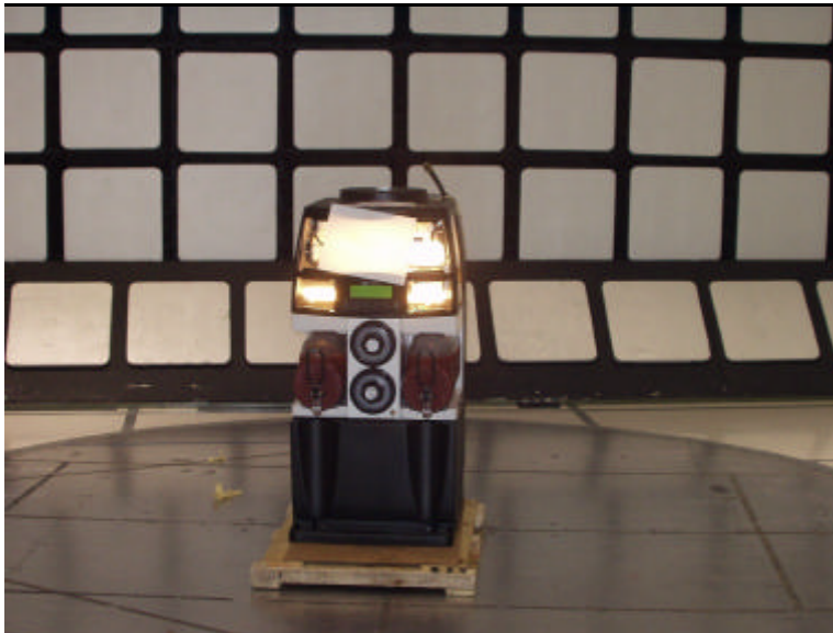
Radiated Emissions & Occupied Band Width (10M Chamber)
