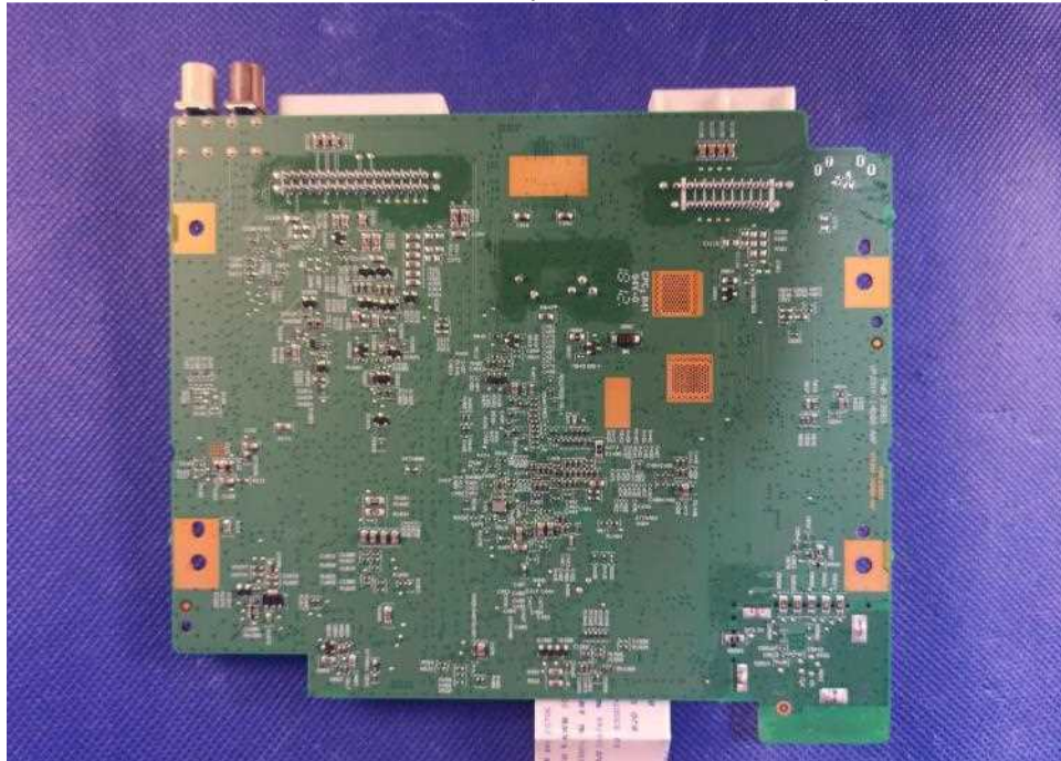
Photo 9 Internal view (R013 PH2-X07 WDAB)
