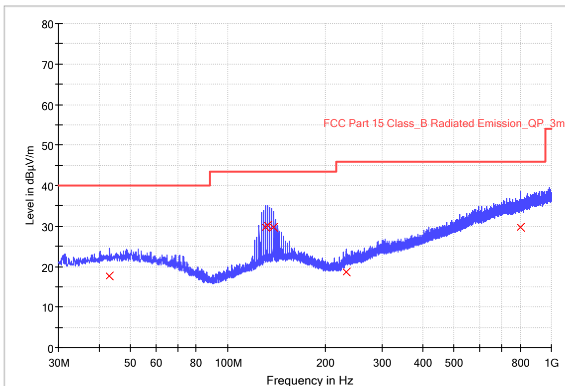
RE_VULB9163_pre_Cont_30-1000
