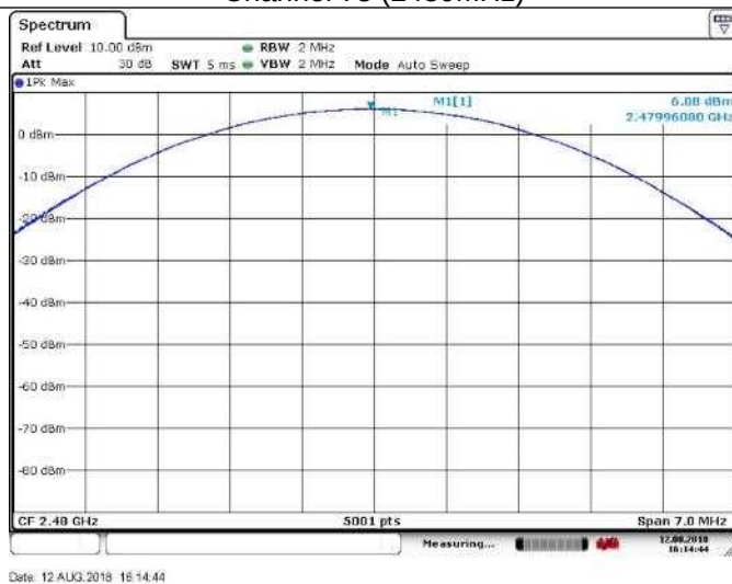
Channel 78 (2480MHz)
