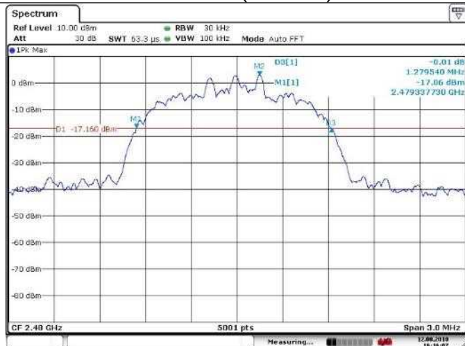
Channel 78 (2480MHz)
