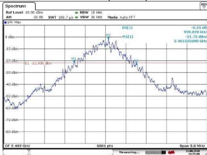
Channel 00 (2402MHz)
