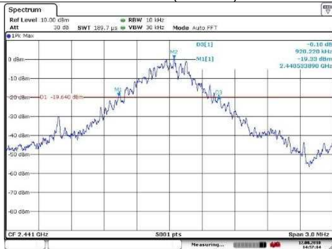
Channel 39 (2441MHz)
