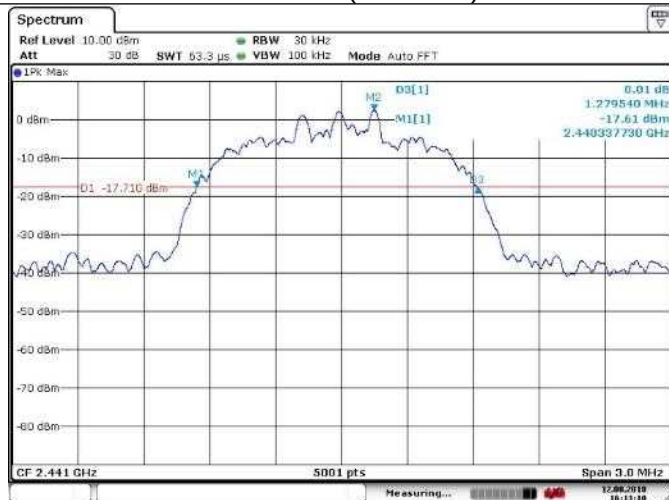
Channel 39 (2441MHz)
