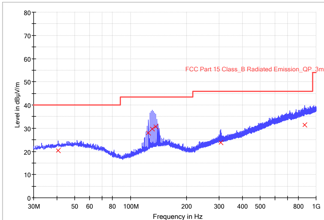
RE_VULB9163_pre_Cont_30-1000
