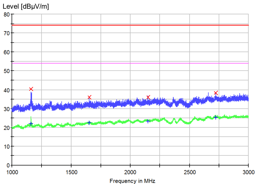
Figure 8: Spectral Diagrams and measurement results, 1 GHz-3 GHz, vertical polarization for mode 2
