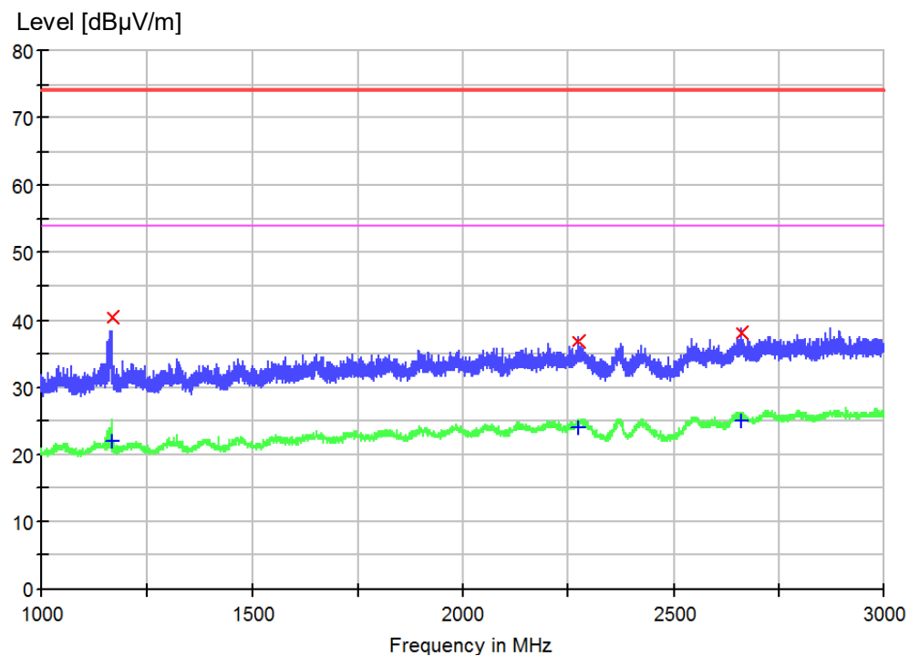
Figure 6: Spectral Diagrams and measurement results, 1 GHz-3 GHz, vertical polarization for mode 1
