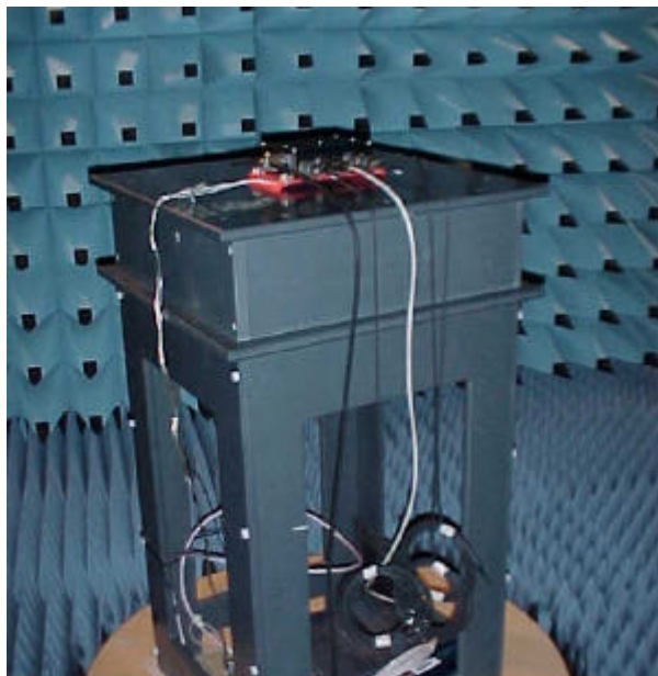
Radiated spurious emission 1 – 26 GHz
