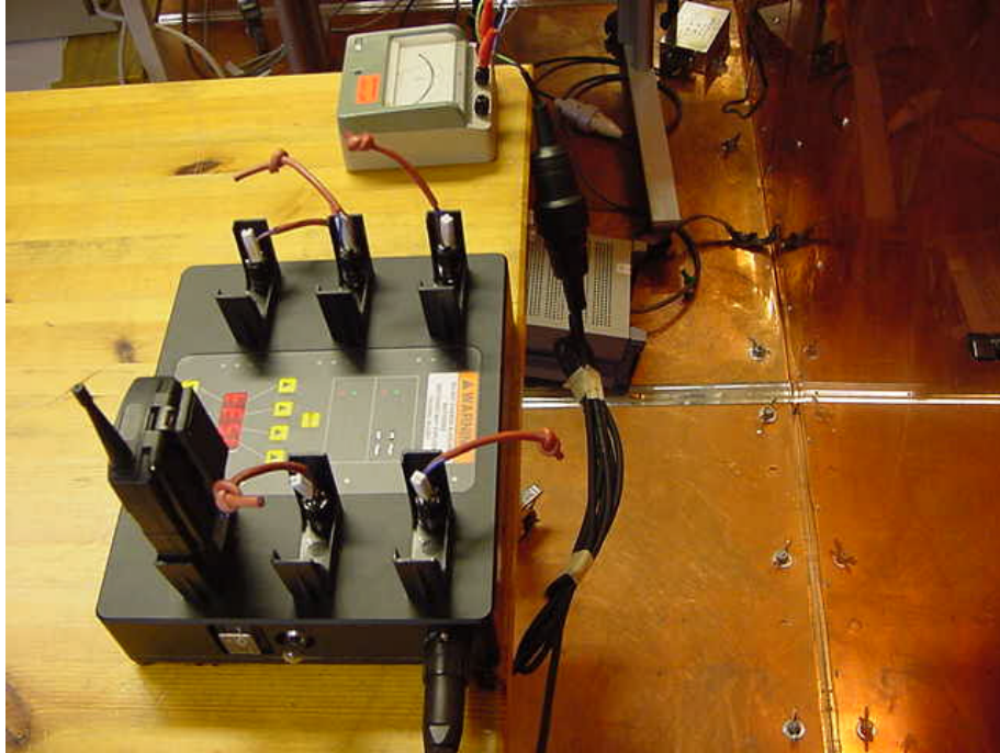
Conducted spurious emission
