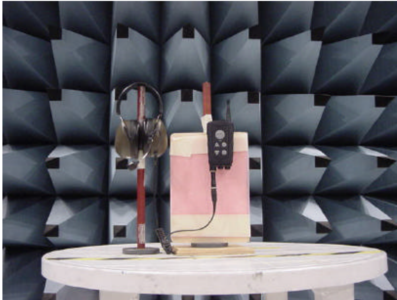
Radiated spurious emission 30 – 1000 MHz
