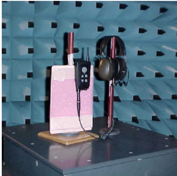
Radiated spurious emission 1 – 26 GHz
