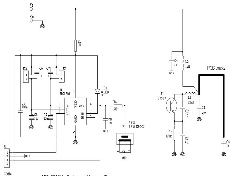
433.92MHz 2 channel transmitter Board: Larco Tx1
