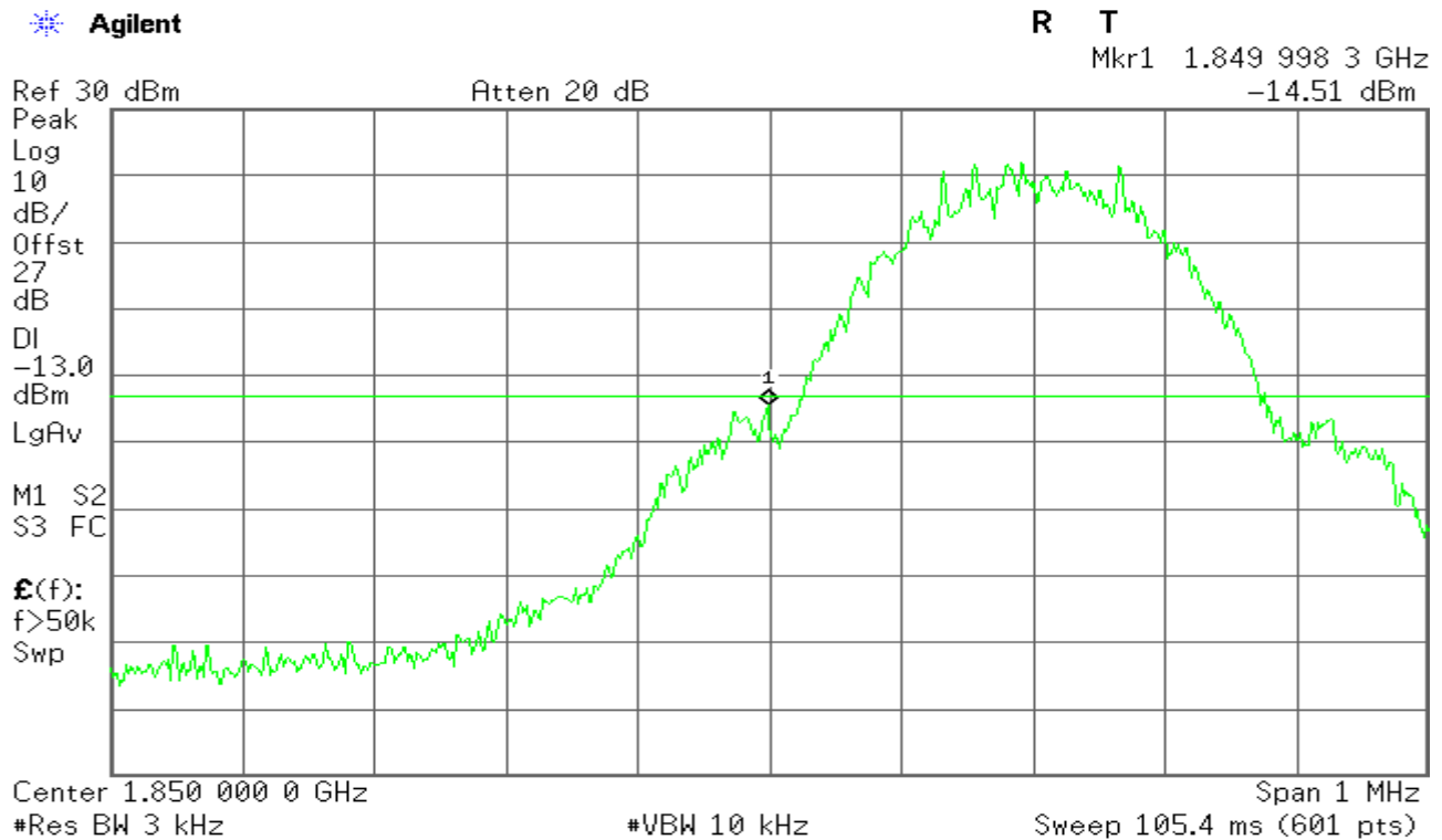
Figure 8-1: Band Edge emissions –CH Low
