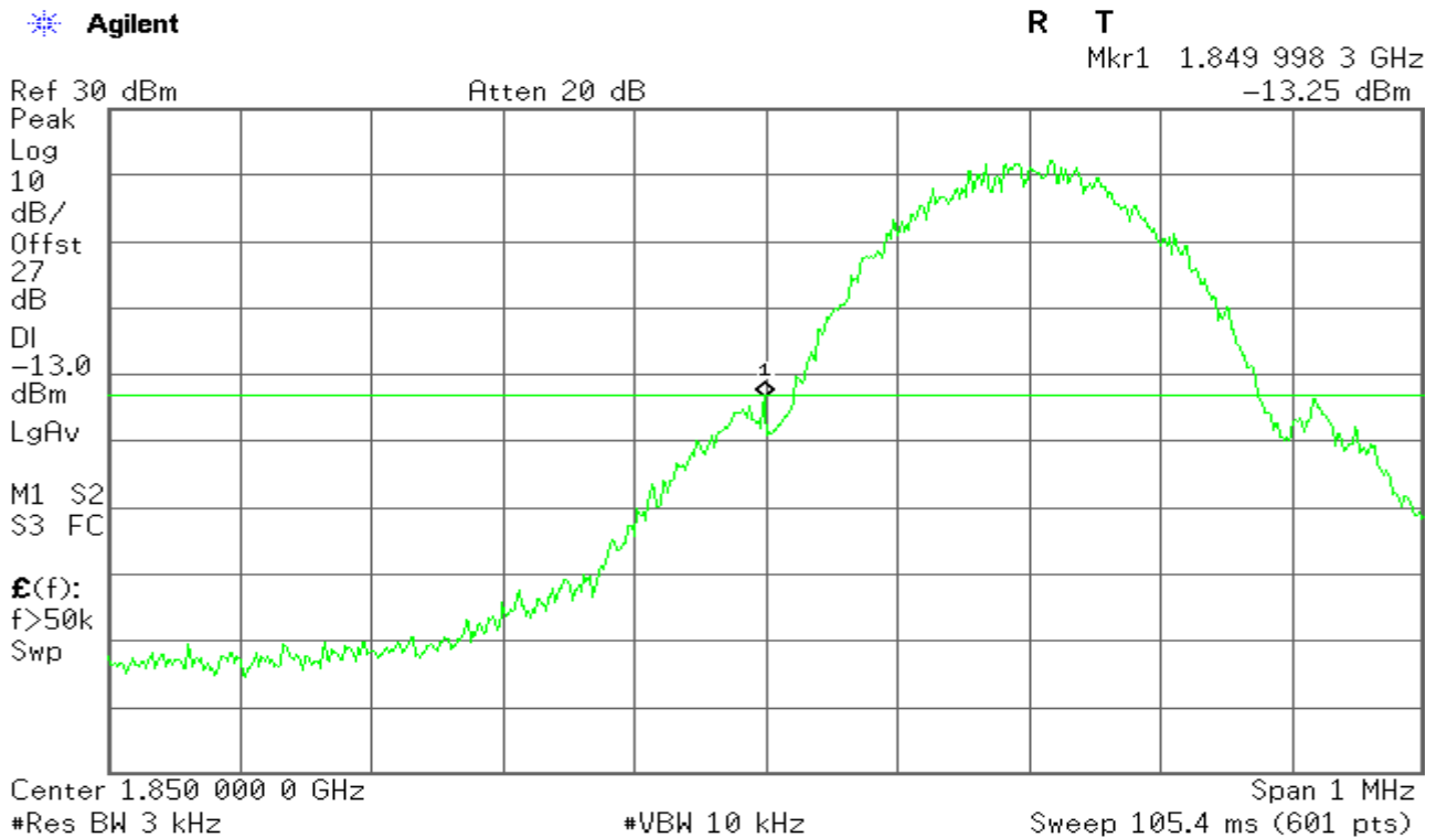
Figure 4-1: Band Edge emissions – GSM CH Low
