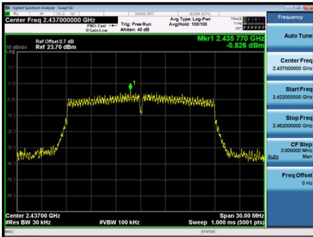
(Plot 4.4.3 B: Channel 6: 2437MHz @ 802.11n HT20)
