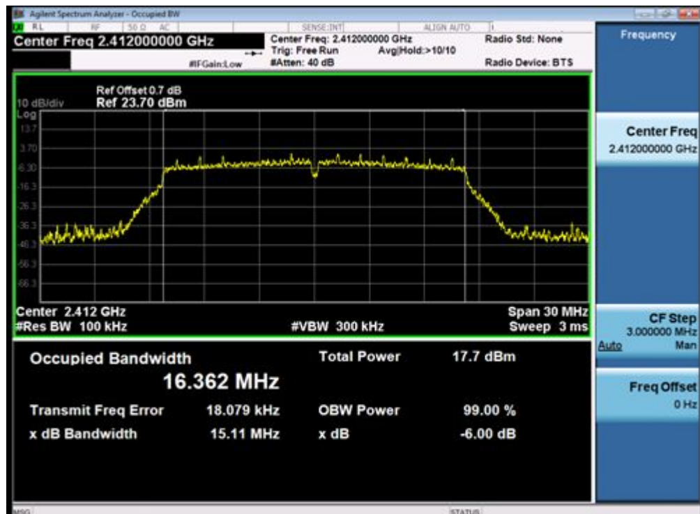
(Plot 4.7.2 A: Channel 1: 2412MHz @ 802.11g)
