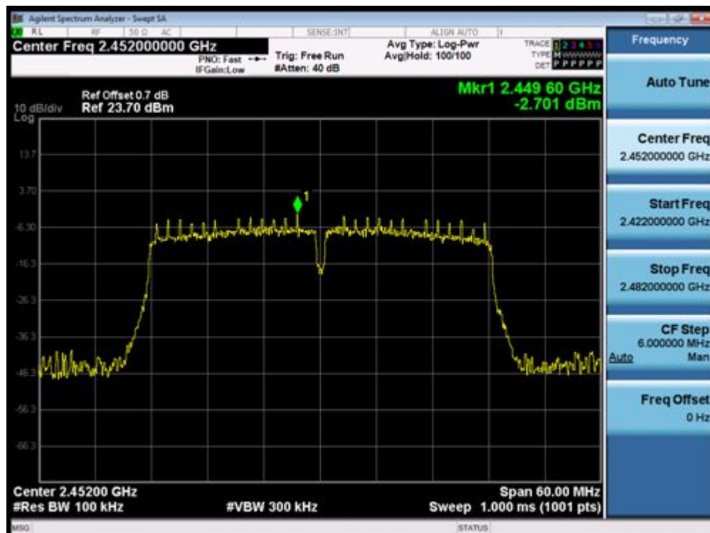
(Plot 4.6.4 C1: Channel 9 : 2452MHz @ 802.11n HT40)
