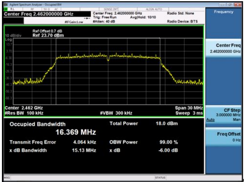
(Plot 4.7.2 C: Channel 11: 2462MHz @ 802.11g)
