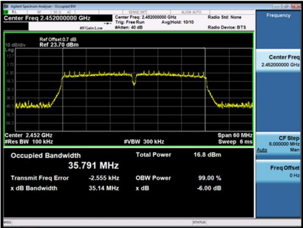
(Plot 4.7.4 C: Channel 9: 2452MHz @ 802.11n HT40MHz)
