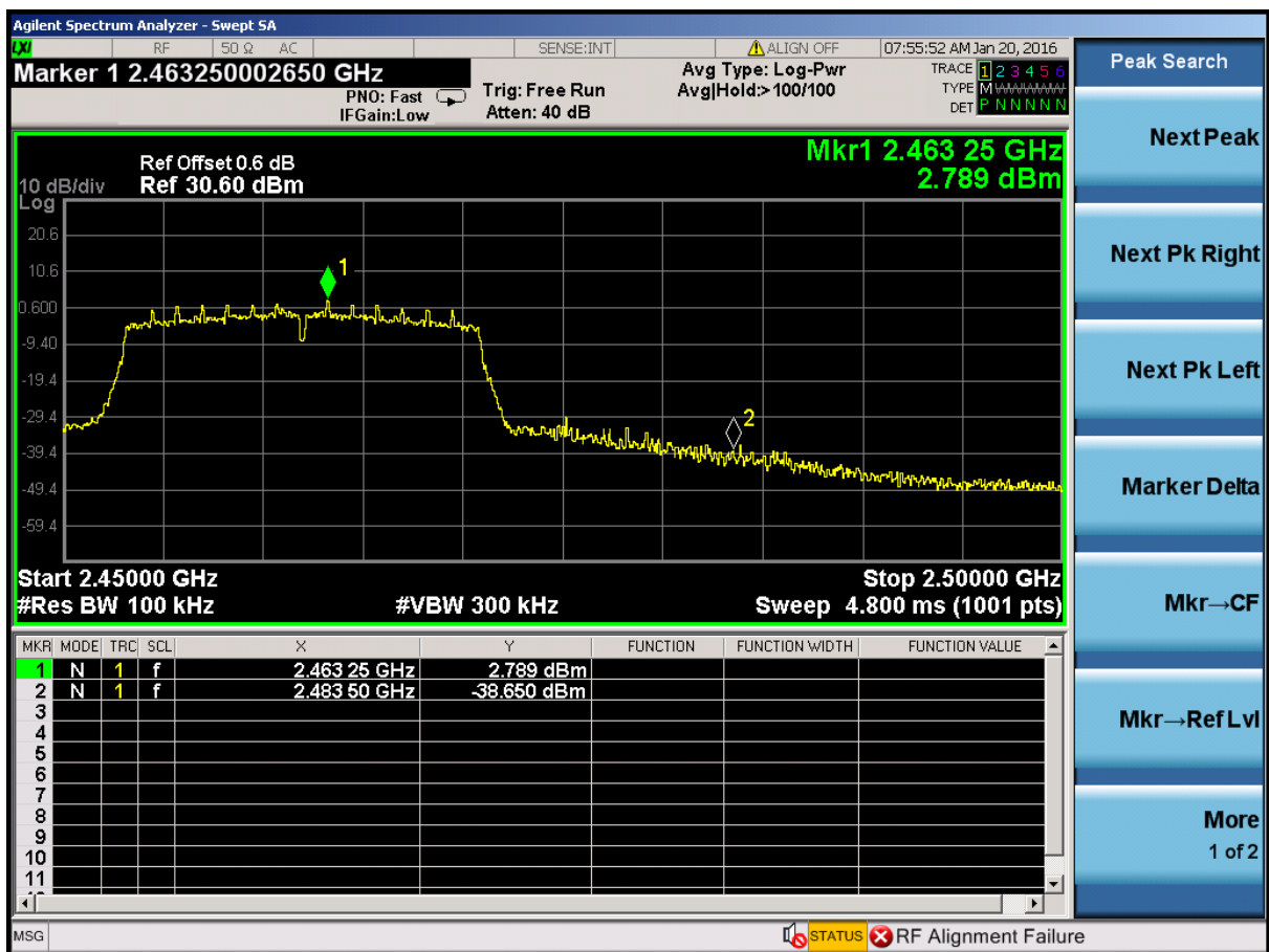
(Plot 4.5.3 D2: Right Band edge @ 802.11n HT20)
