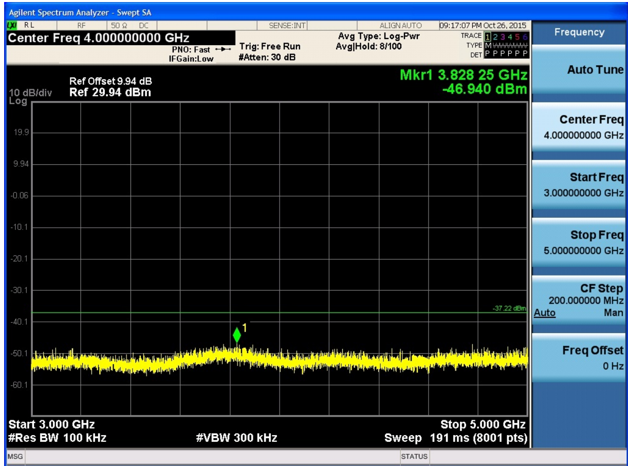
(Plot 4.6.4 B3: Channel 6: 2437MHz @ 802.11n HT40)
