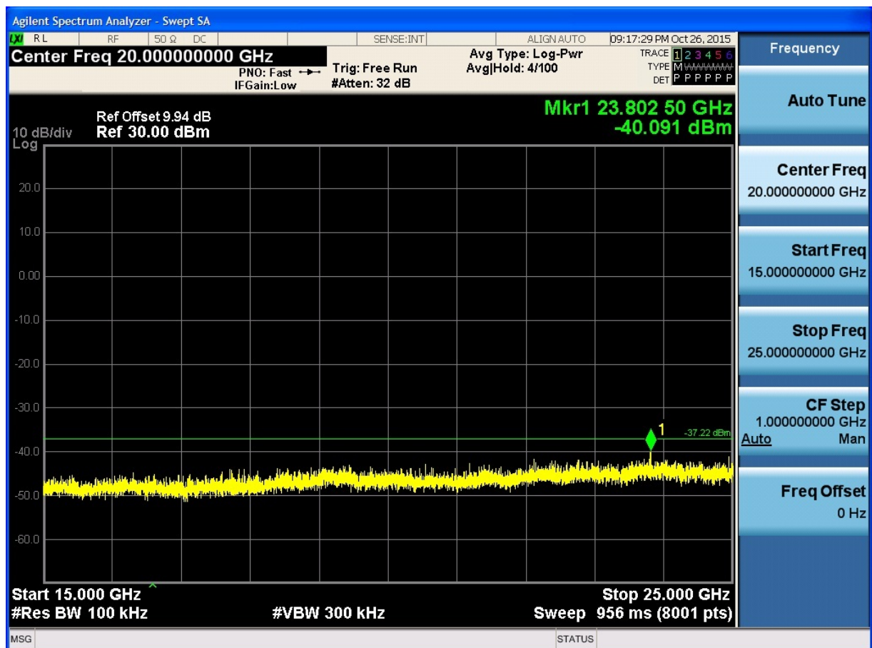
(Plot 4.6.4 B6: Channel 6: 2437MHz @ 802.11n HT40)
