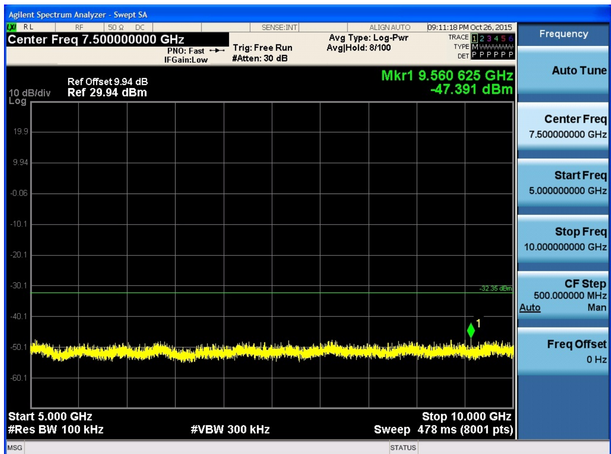
(Plot 4.6.3 C4: Channel 11: 2462MHz @ 802.11n HT20)
