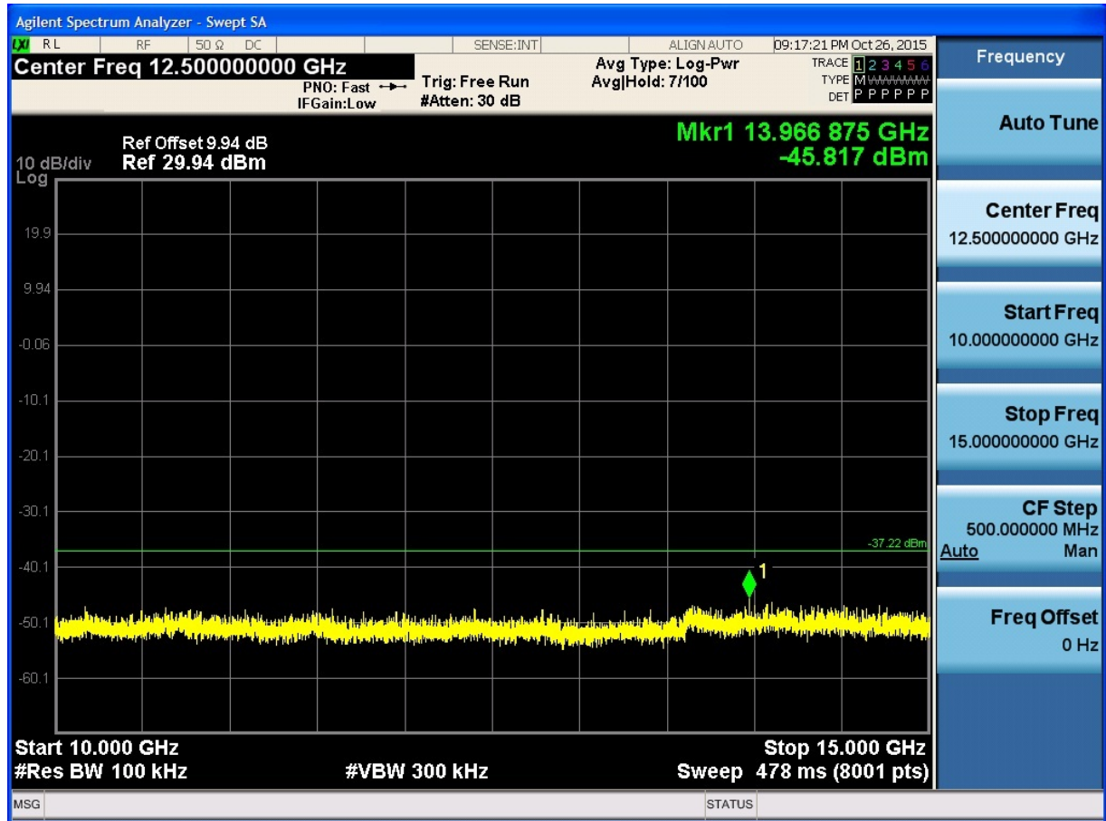
(Plot 4.6.4 B5: Channel 6: 2437MHz @ 802.11n HT40)
