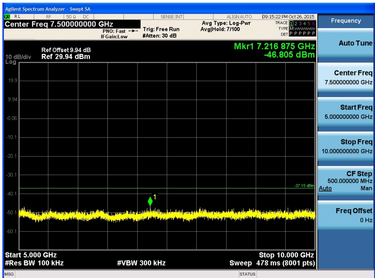
(Plot 4.6.4 A4: Channel 3: 2422MHz @ 802.11n HT40)
