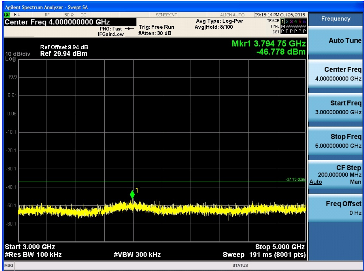
(Plot 4.6.4 A3: Channel 3: 2422MHz @ 802.11n HT40)
