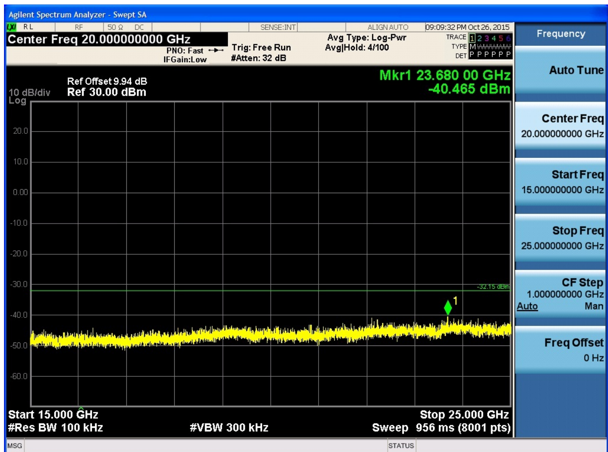
(Plot 4.6.3 B6: Channel 6: 2437MHz @ 802.11n HT20)
