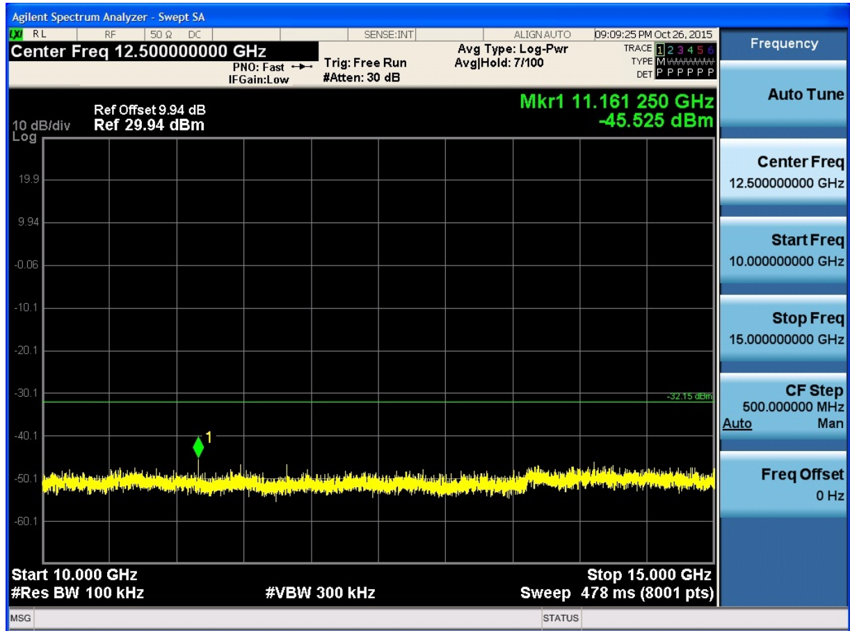
(Plot 4.6.3 B5: Channel 6: 2437MHz @ 802.11n HT20)
