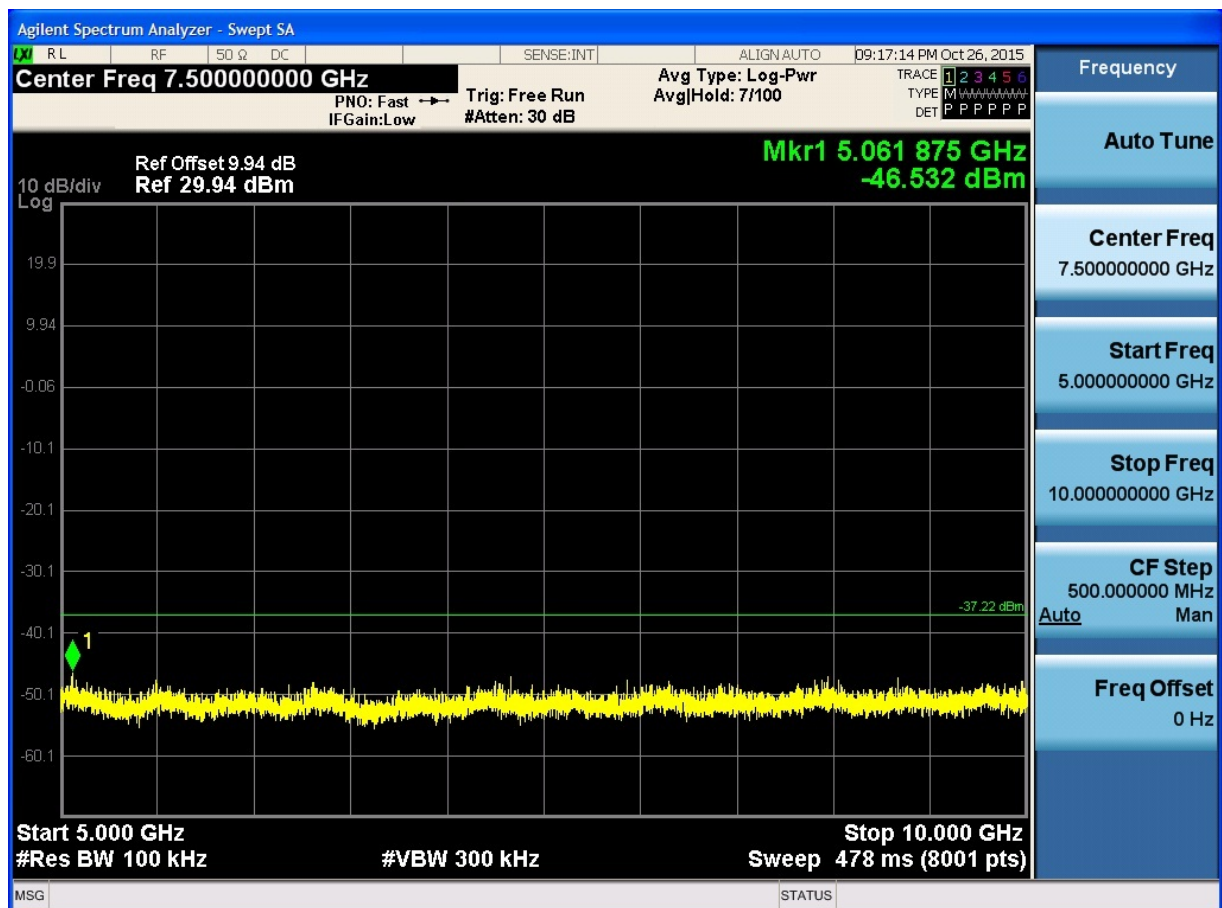
(Plot 4.6.4 B4: Channel 6: 2437MHz @ 802.11n HT40)
