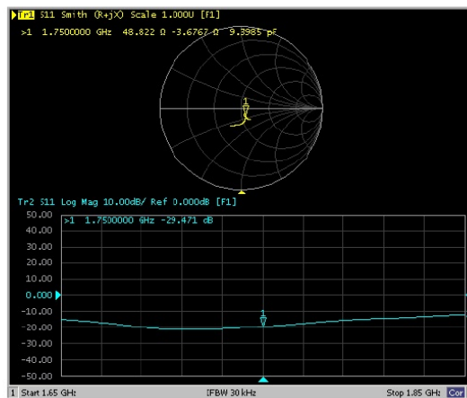
1750MHz Head
