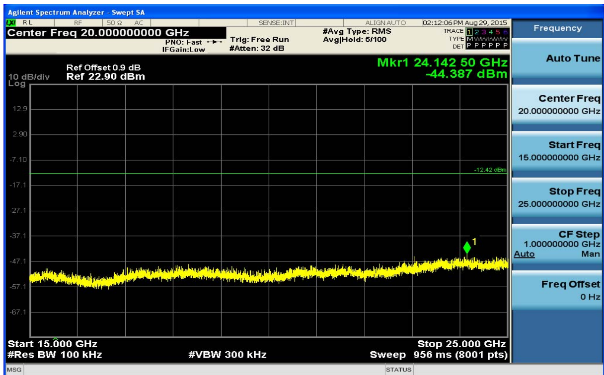
(Plot 4.6.1 B6: Channel 19: 2440MHz @ GFSK)
