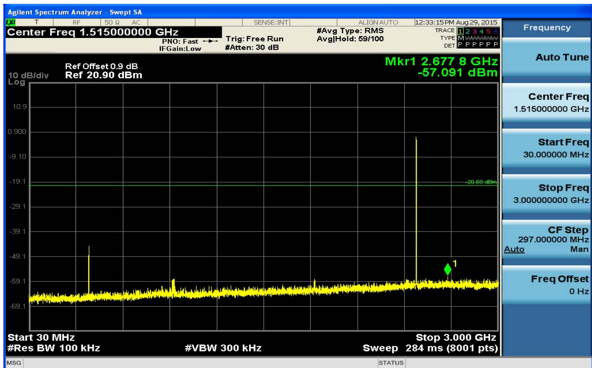
(Plot 4.6.1 C2: Channel 39: 2480MHz @ GFSK)
