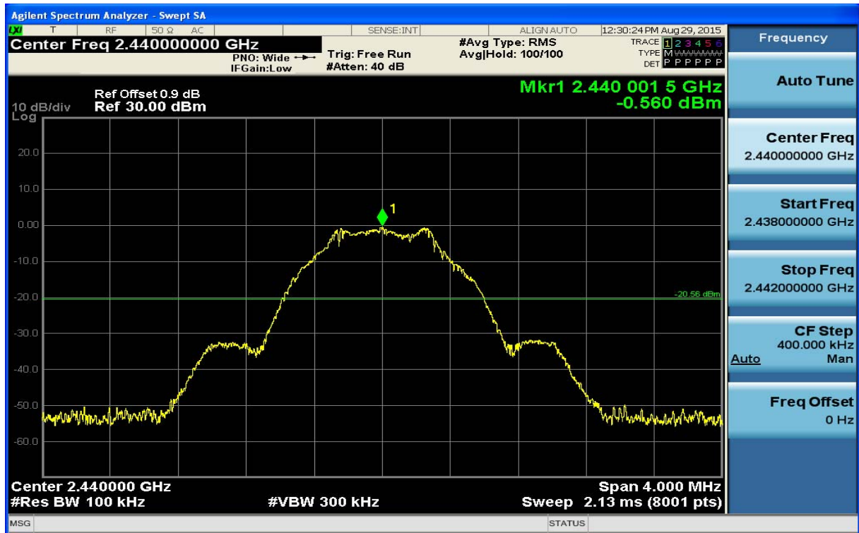
(Plot 4.6.1 B1: Channel 19: 2440MHz @ GFSK)
