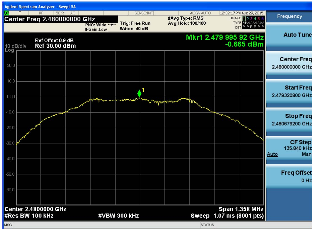
(Plot 4.4.1 C: Channel 39: 2480 MHz @ GFSK
