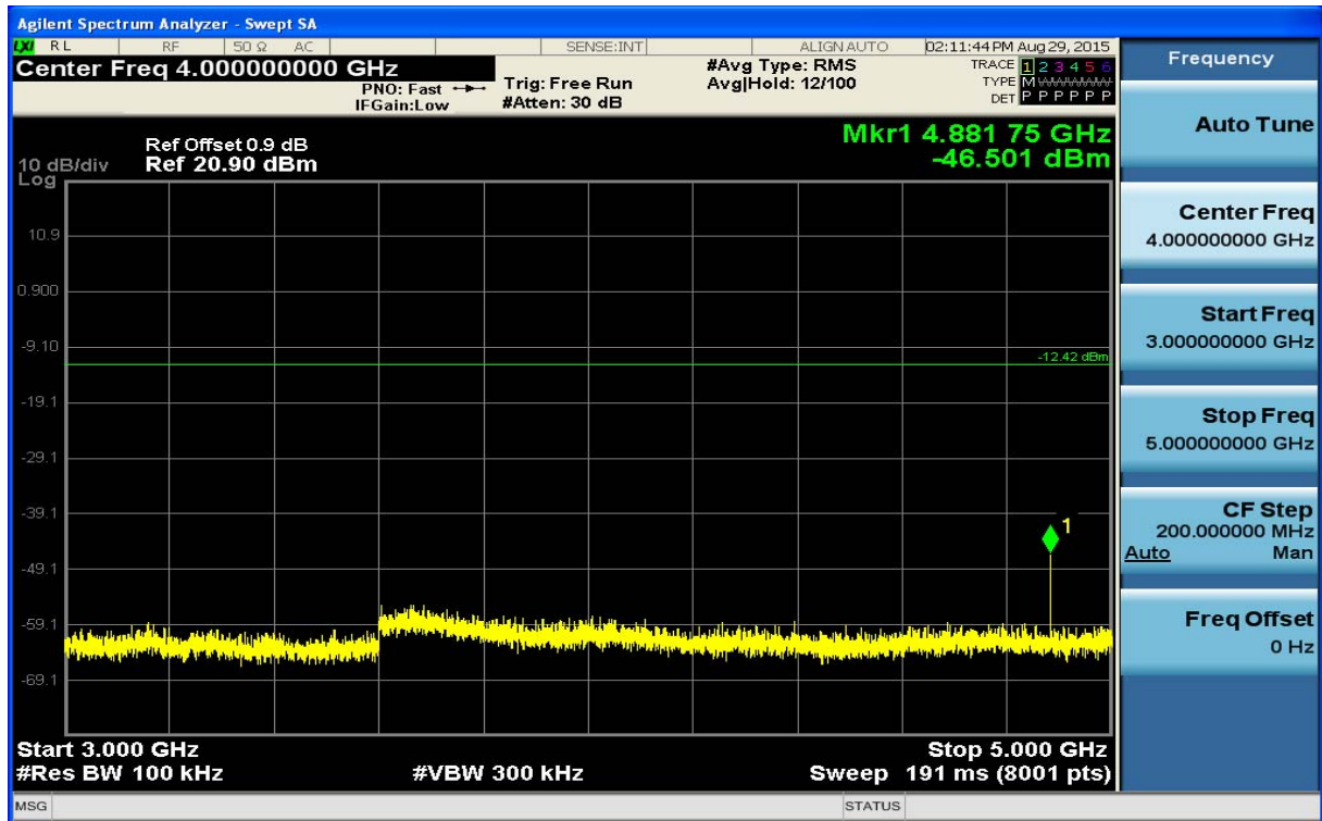
(Plot 4.6.1 B3: Channel 19: 2440MHz @ GFSK)
