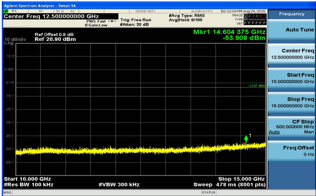
(Plot 4.6.1 C5: Channel 39: 2480MHz @ GFSK)
