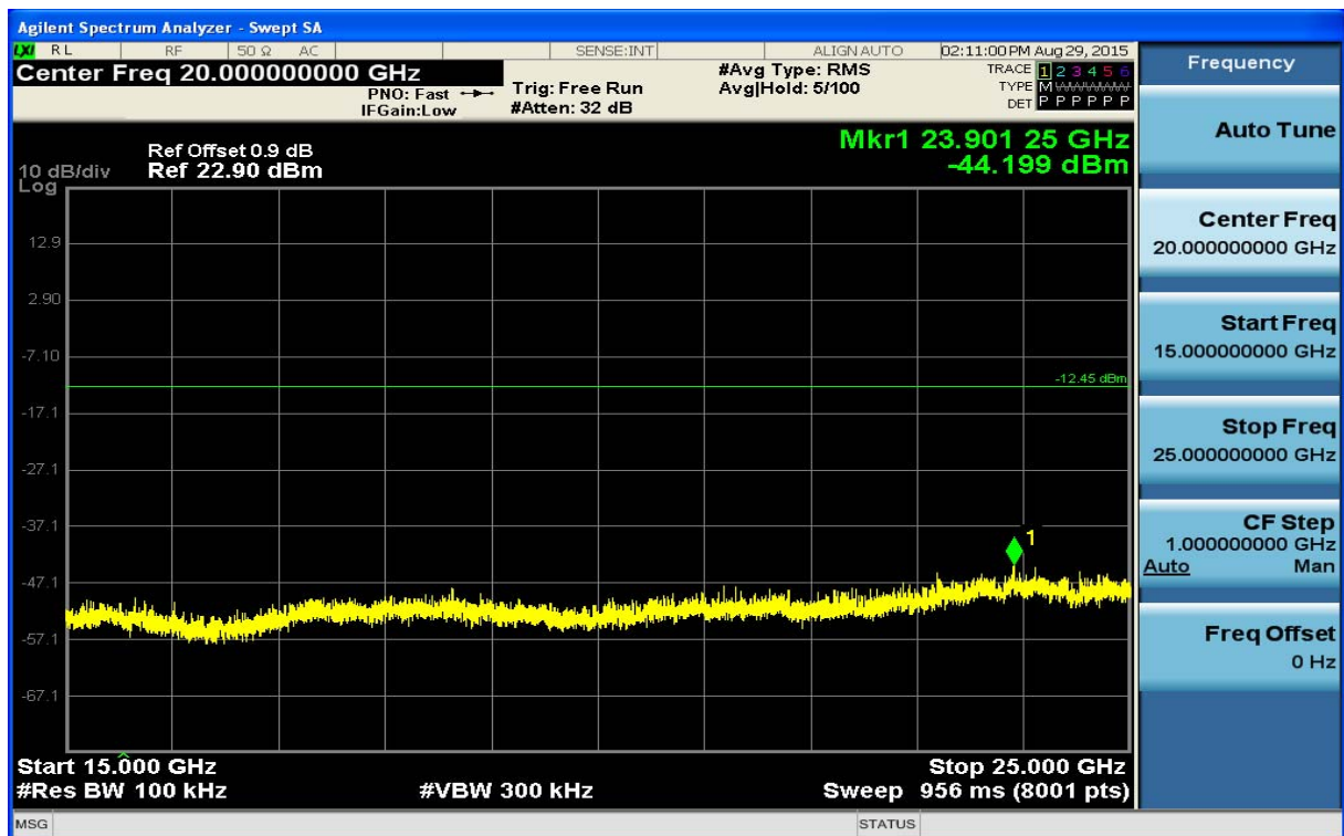
(Plot 4.6.1 A6: Channel 00: 2402MHz @ GFSK)
