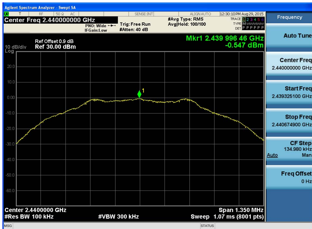
(Plot 4.4.1 B: Channel 19: 2440 MHz @ GFSK)
