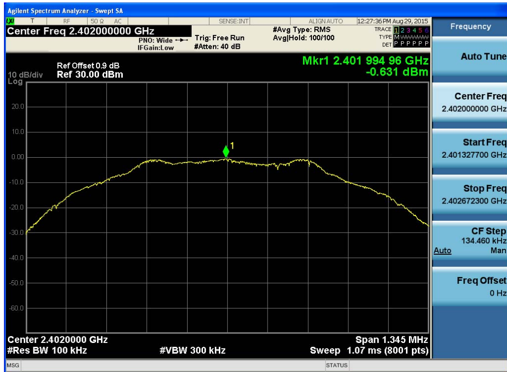
(Plot 4.4.1 A: Channel 00: 2402 MHz @ GFSK)
