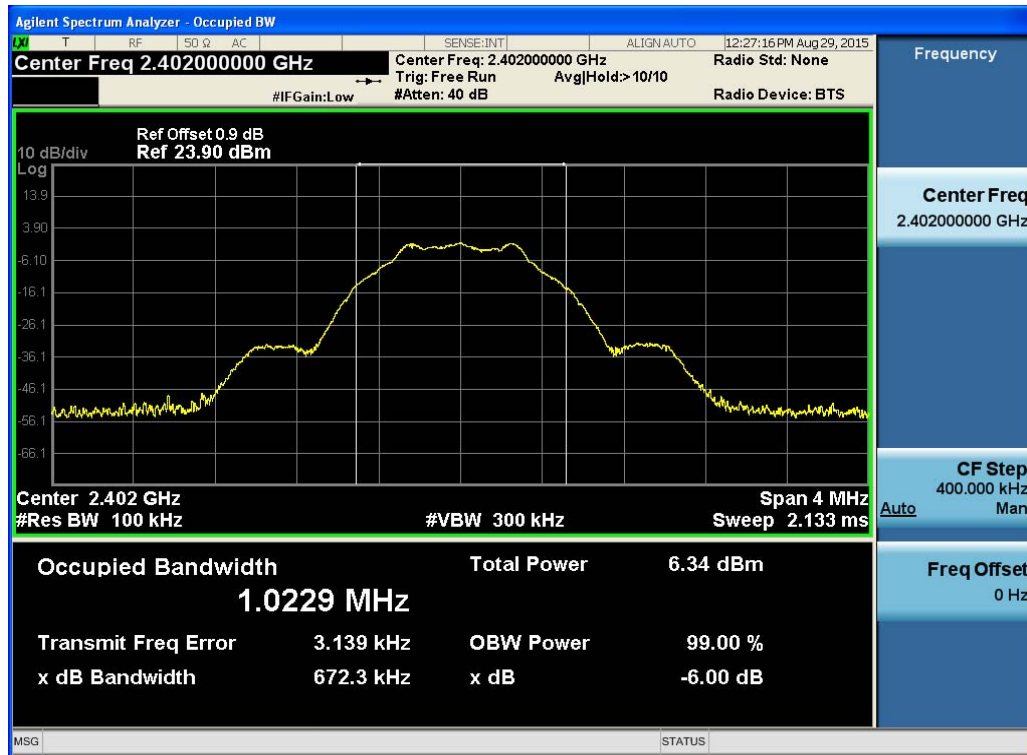
(Plot 4.7.1 A: Channel 00: 2402MHz @ GFSK)
