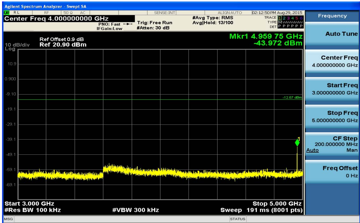
(Plot 4.6.1 C3: Channel 39: 2480MHz @ GFSK)
