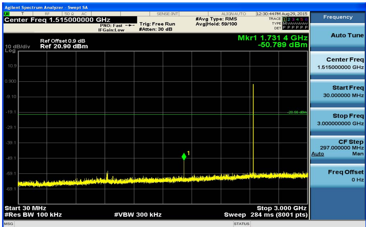
(Plot 4.6.1 B2: Channel 19: 2440MHz @ GFSK)
