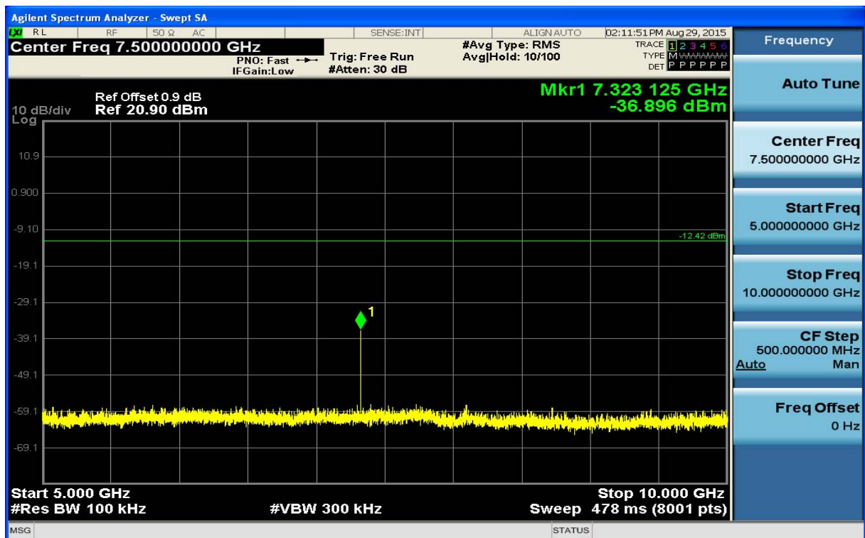
(Plot 4.6.1 B4: Channel 19: 2440MHz @ GFSK)
