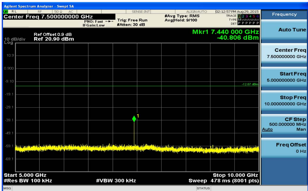
(Plot 4.6.1 C4: Channel 39: 2480MHz @ GFSK)
