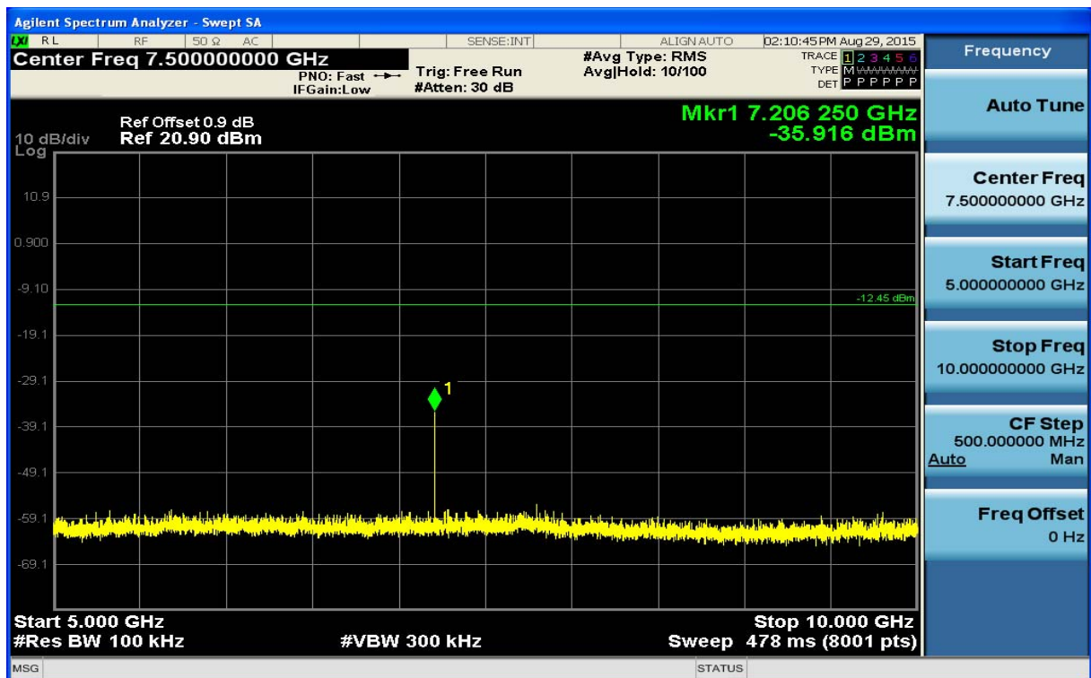
(Plot 4.6.1 A4: Channel 00: 2402MHz @ GFSK)
