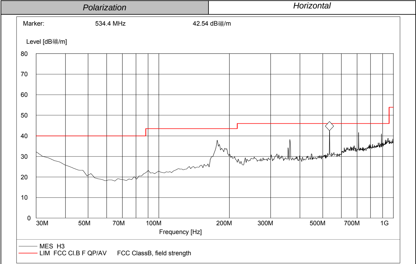
30MHz-1GHz
