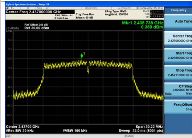
Channel 6 / 2437 MHz
