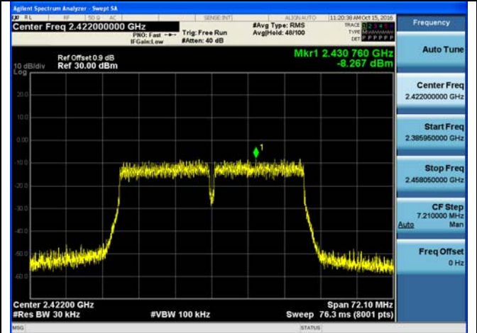
Channel 3 / 2422 MHz
