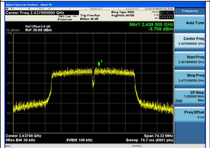
Channel 6 / 2437 MHz
