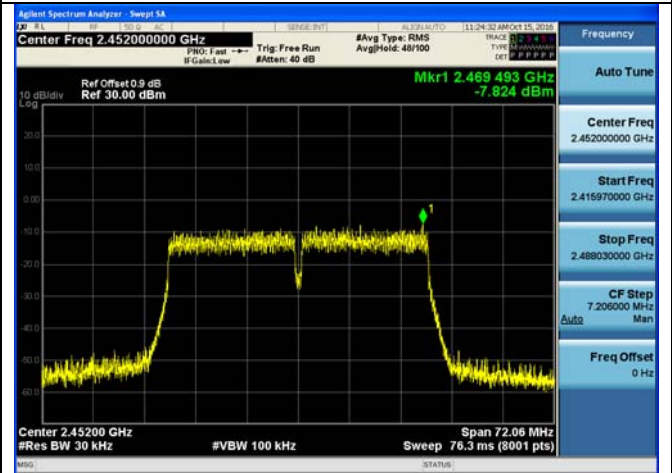
Channel 9 / 2452 MHz
