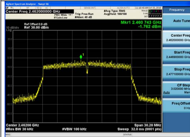
Channel 11 / 2462 MHz
