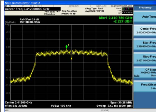
Channel 1 / 2412 MHz
