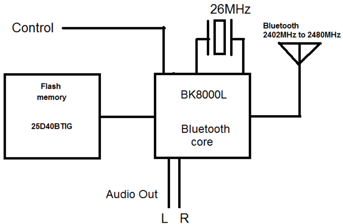
F-6188 Bluetooth Module Block Diagram
