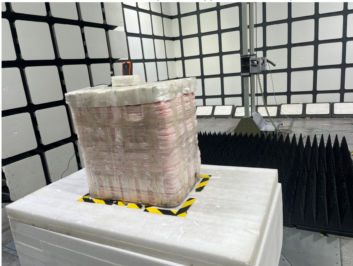
Radiated Emissions View (Above 1GHz) (Model: WM-5000P4D)
