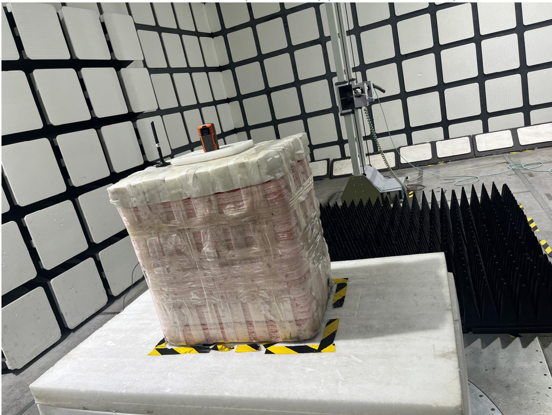
Radiated Emissions View (Above 1GHz) (Model: WM-5000L4D)
