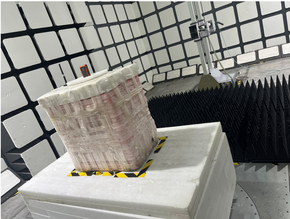
Radiated Emissions View (Above 1GHz) (Model: WM-5000P4)
