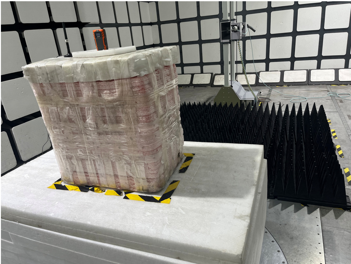
Radiated Emissions View (Above 1GHz) (Model: WM-5000L4)
