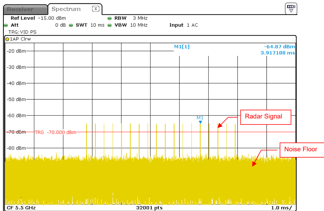
Radar Signal 3
