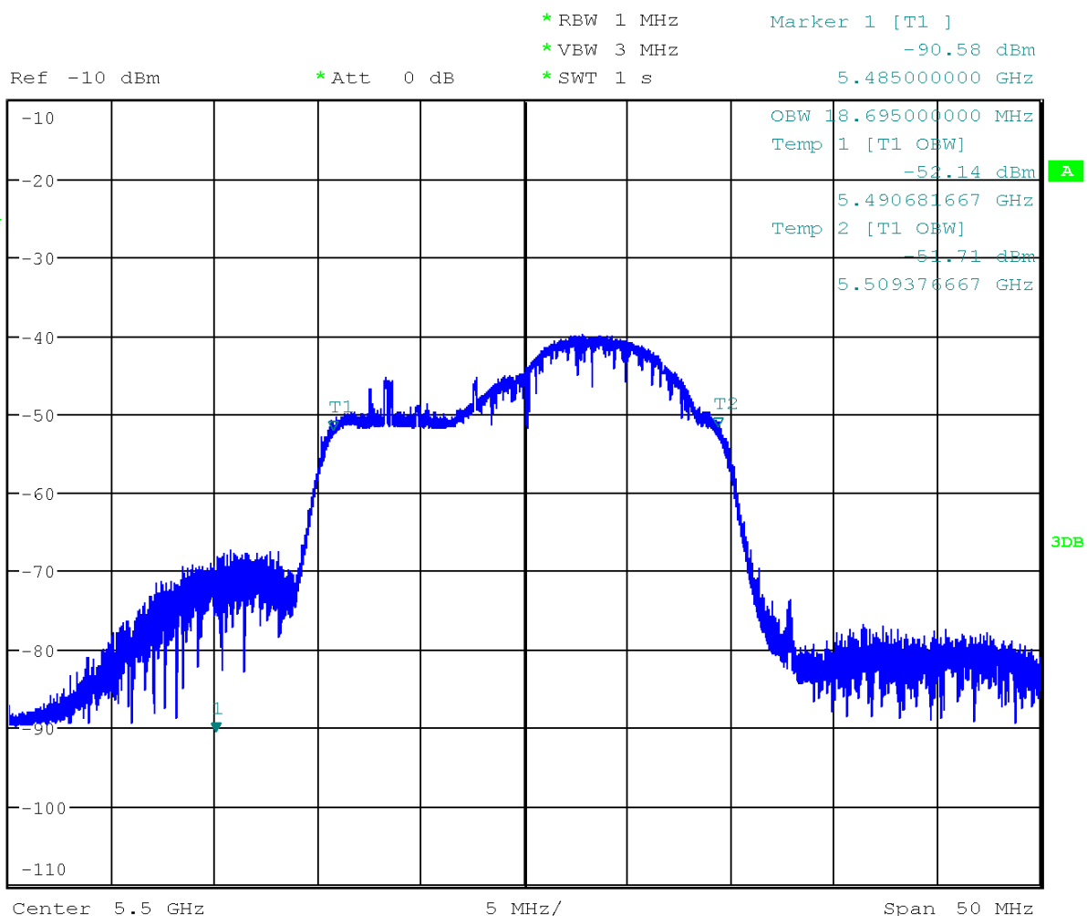
U-NII 99% Channel bandwidth
