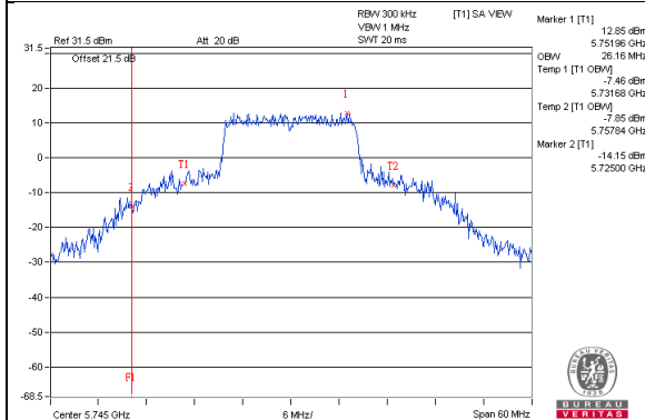
802.11ac(VHT20)_Chain0 / CH149
