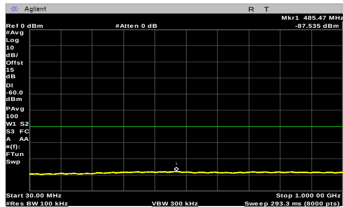
Figure 7: Conducted Spurious Emissions - 30-1000 MHz
