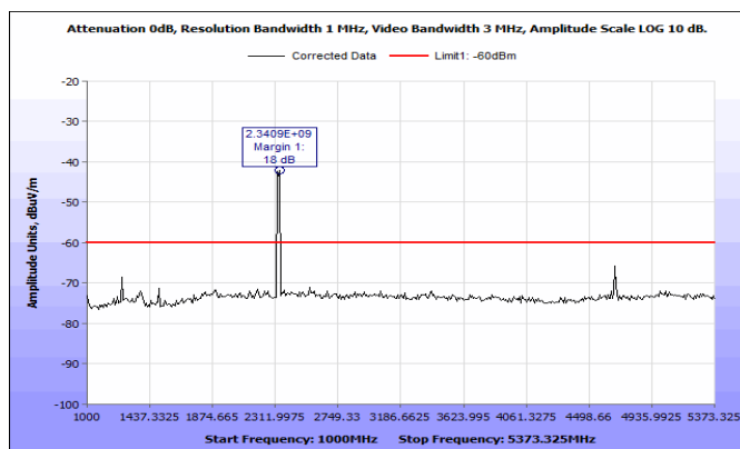
Figure 19: Cabinet Spurious Emissions, TX ON, 1-6 GHz, Vertical.
