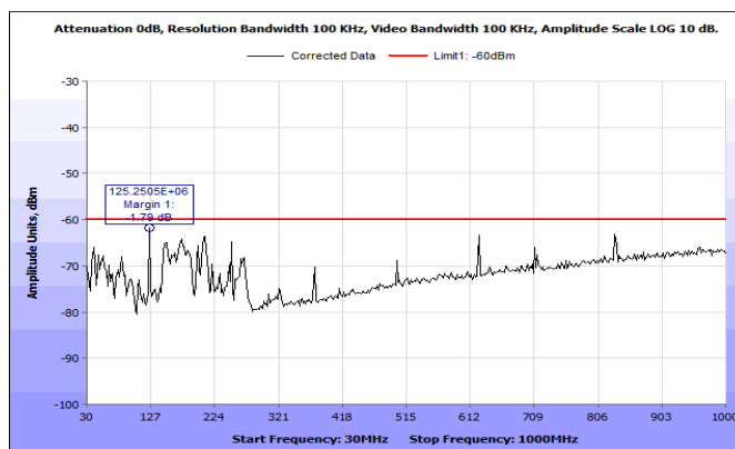
Figure 16: Cabinet Spurious Emissions, TX OFF, 30-1000 MHz.
