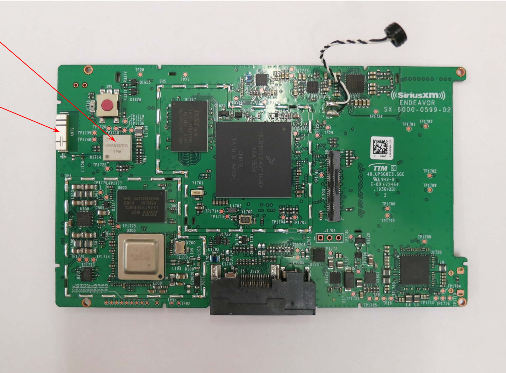
BT/WiFi Module and Antenna Locations on Endeavor/Tour PCB
