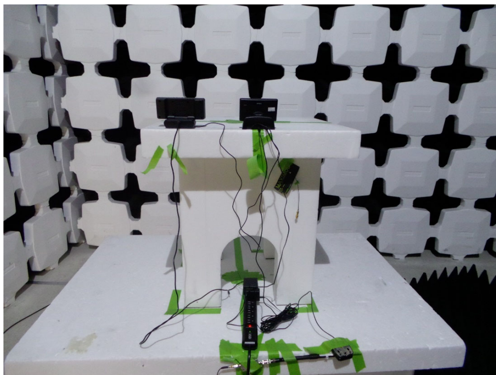
Test Configuration 4: Radiated Emissions 1-26.5GHz (rear)
