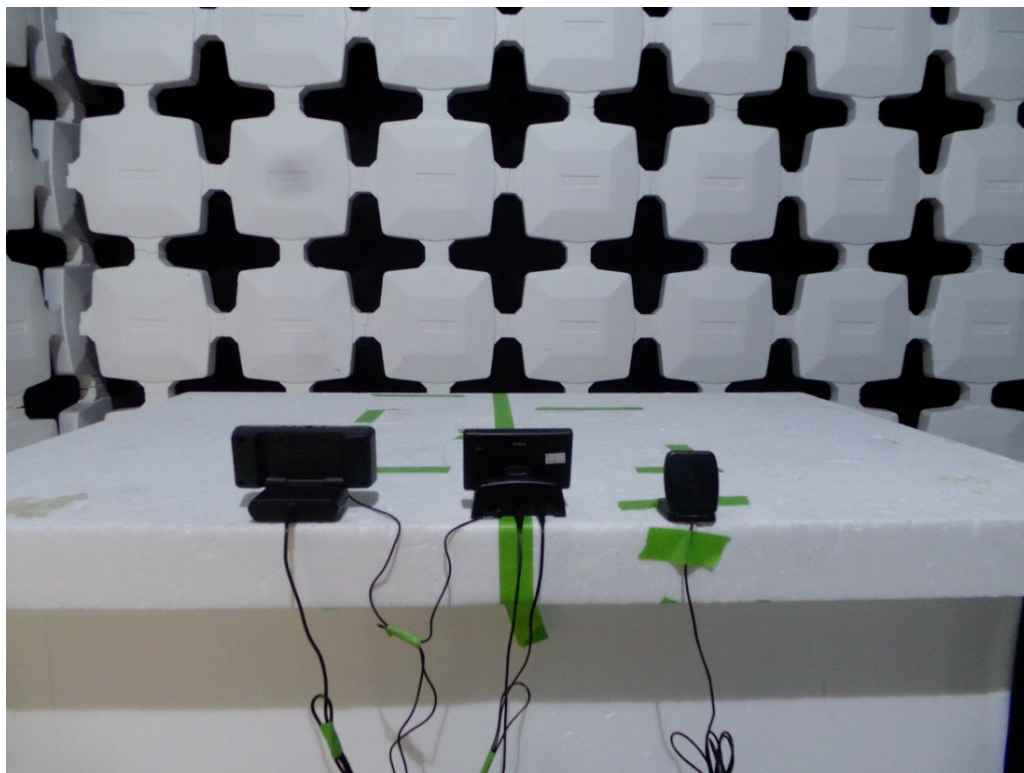
Test Configuration 3: Radiated Emissions 30MHz-1GHz (rear)
