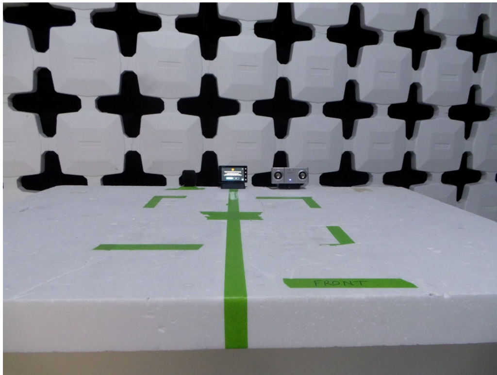
Test Configuration 3: Radiated Emissions 30MHz-1GHz (front)
