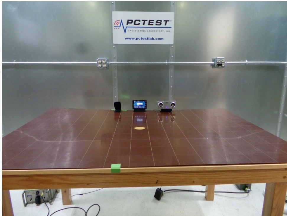
Test Configuration 1: Conducted Emissions, Endeavor with Home Cradle (front)
