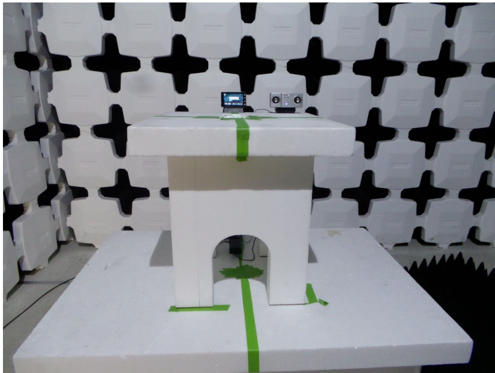
Test Configuration 4: Radiated Emissions 1-26.5GHz (front)
