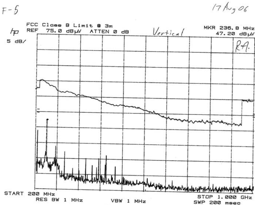
Figure 40 200MHz to 1GHz Vertical (FM)
