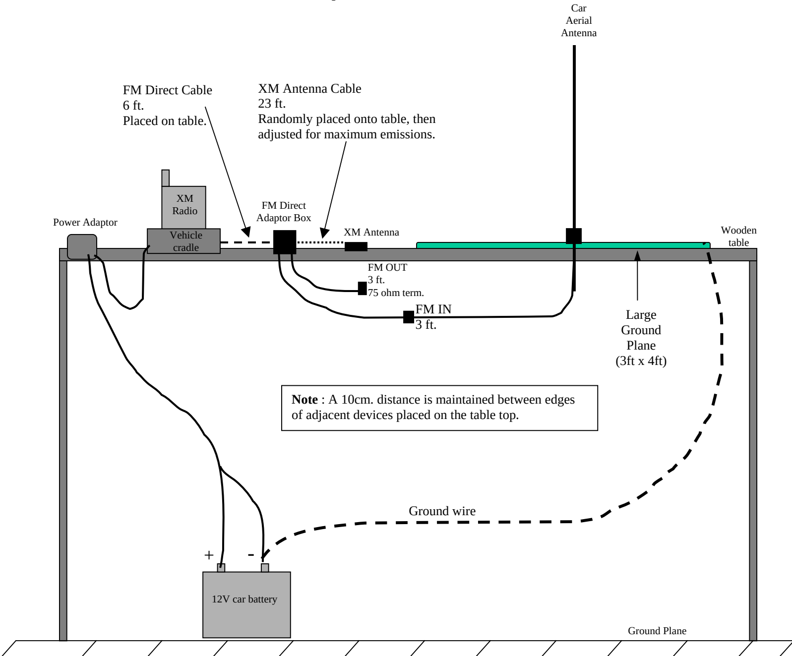
Diagram 2 : FM Direct Adapter Radiated Emissions Setup
