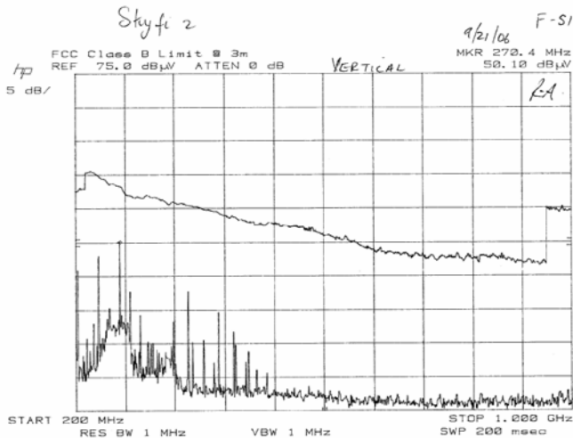
Figure 16 200 MHz to 1000 MHz Vertical FM Programmed to 88.1 MHz
