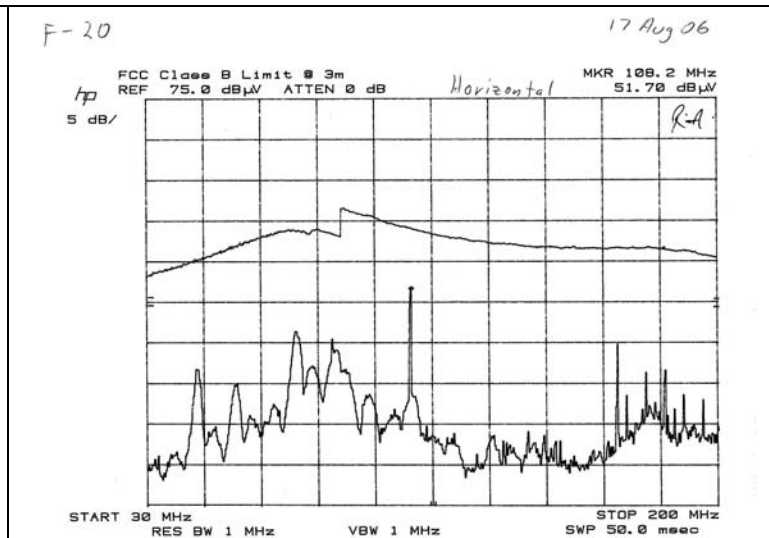
Figure 11 30MHz to 200MHz Horizontal (FM programmed to 107.9MHz)
