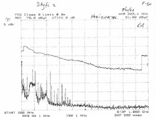
Figure 17 200 MHz to 1000 MHz Horizontal FM Programmed to 88.1 MHz
