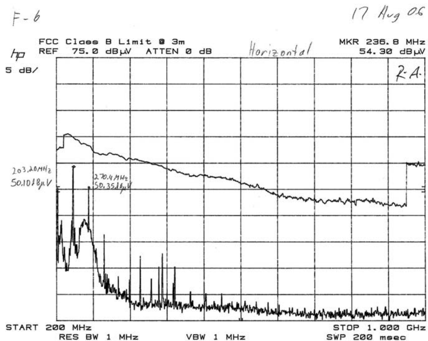
Figure 41 200MHz to 1GHz Horizontal (FM programmed to 88.1MHz)
