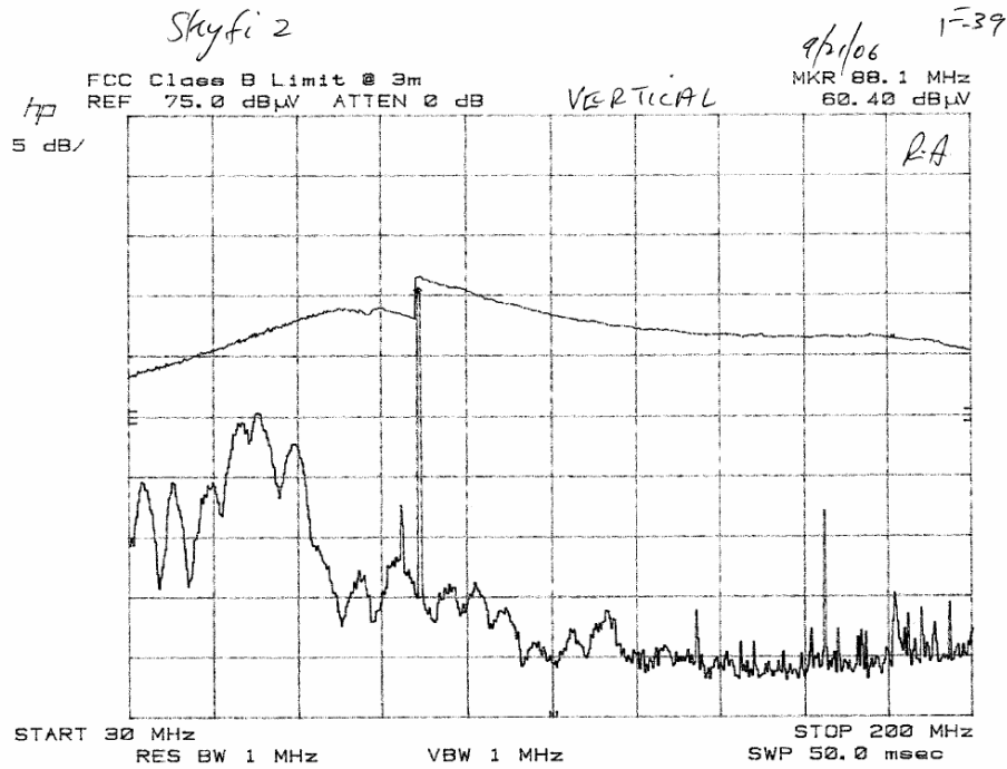
Figure 46 30MHz to 200MHz Vertical (FM programmed to 88.1MHz)
