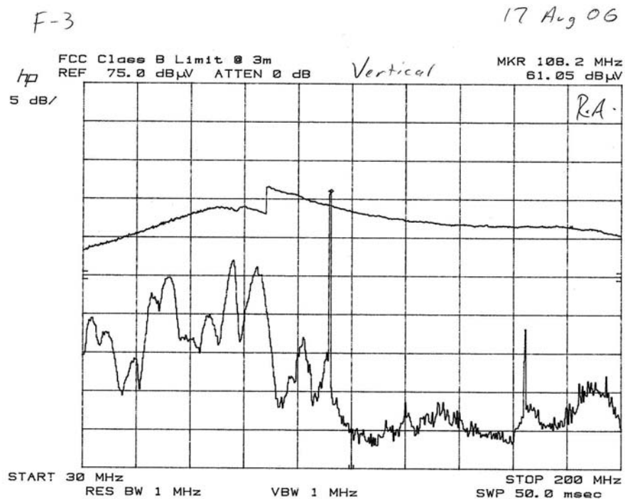
Figure 42 30MHz to 200MHz Vertical (FM programmed to 107.9MHz)
