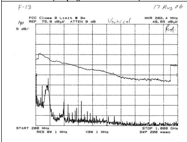
Figure 24 200MHz to 1GHz Vertical (FM programmed to 88.1MHz)
