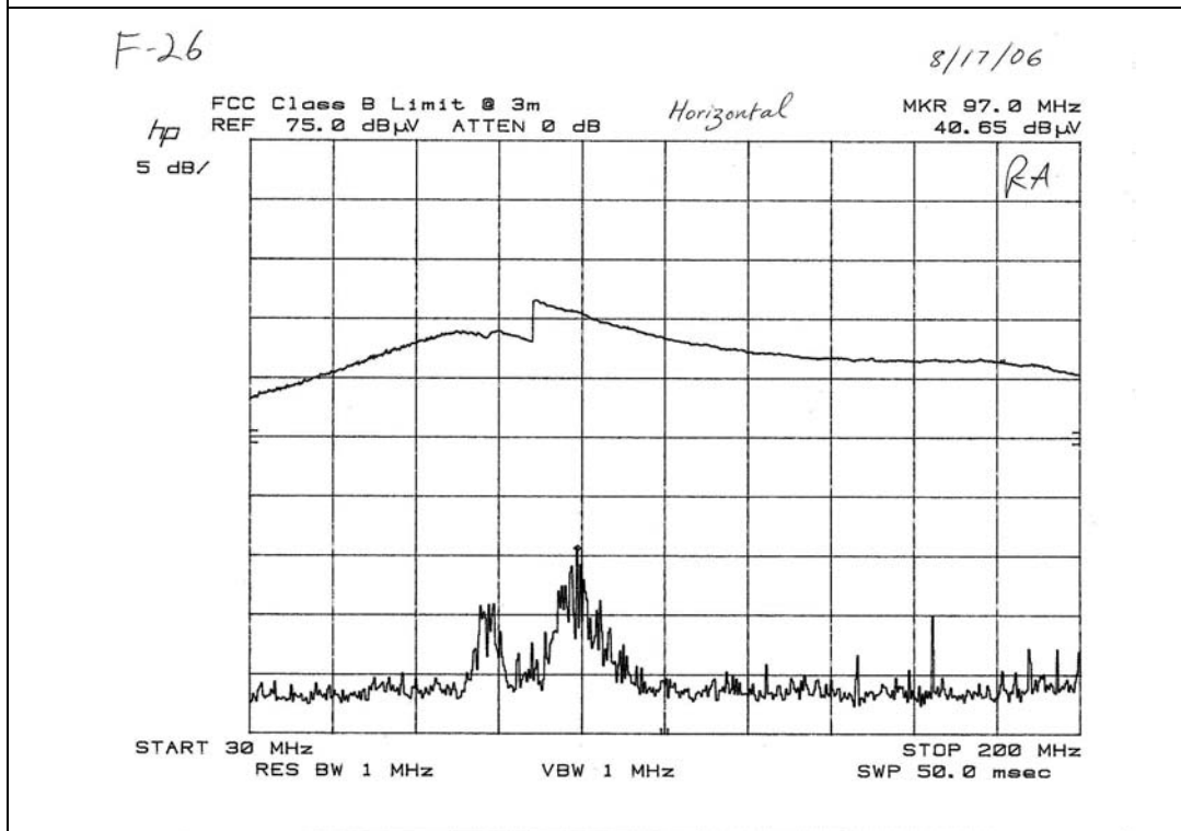
FIGURE 3: Radiated Emission 30 – 200 MHz Horizontal Polarization
