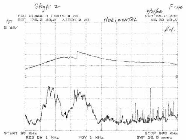
Figure 15 30 MHz to 200 MHz Horizontal FM Programmed to 88.1 MHz
