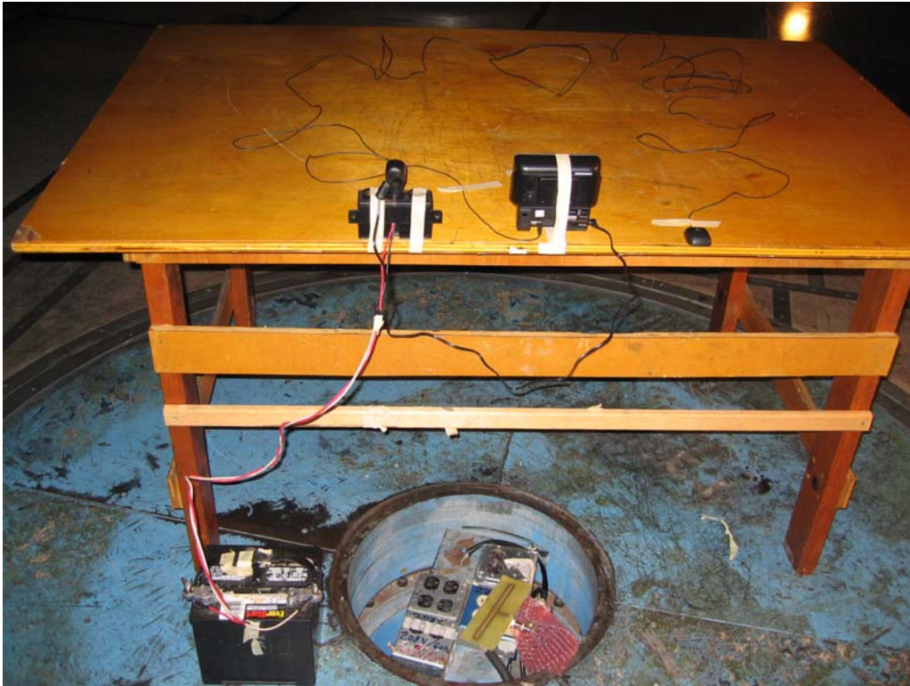
Photograph 5: XM Antenna Only – Radiated Emissions Setup
