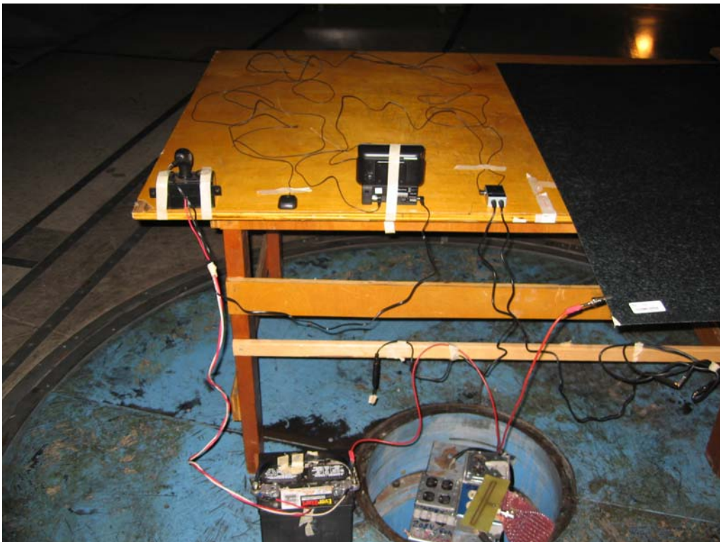
Photograph 4: FM Direct Adapter Radiated Emissions Setup
