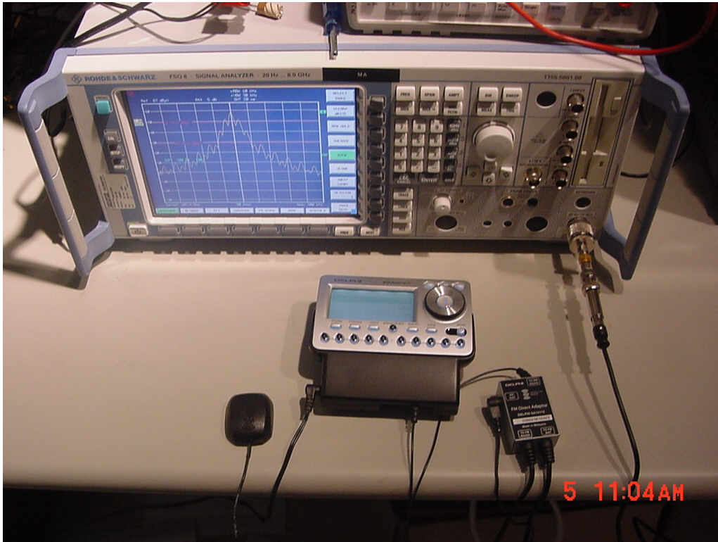
Photograph 13: Occupied Bandwidth Setup
