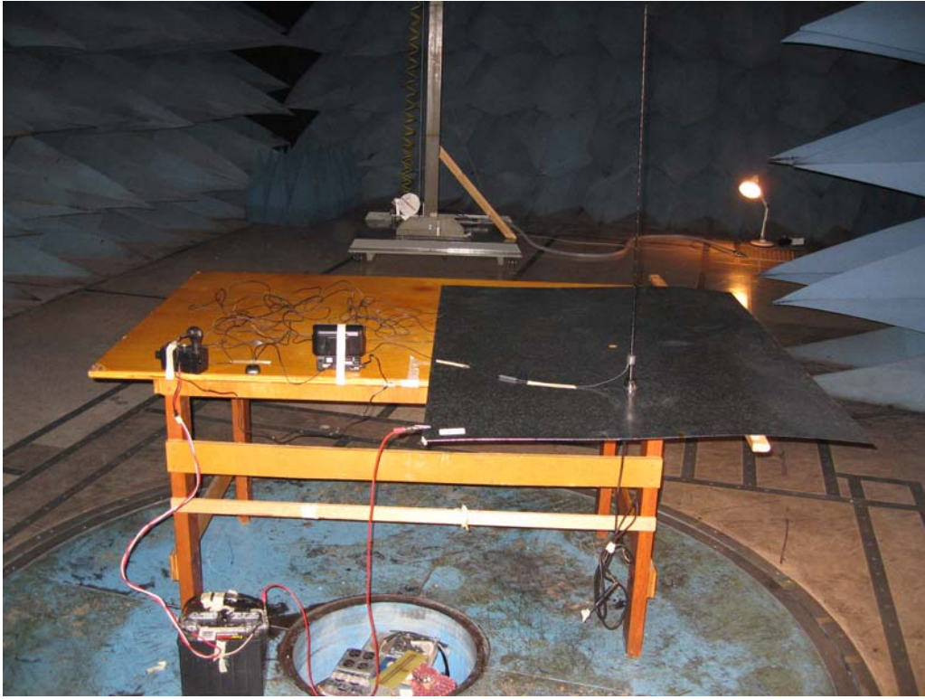
Photograph 6: Intentional Radiator – FM Aerial Antenna Setup
