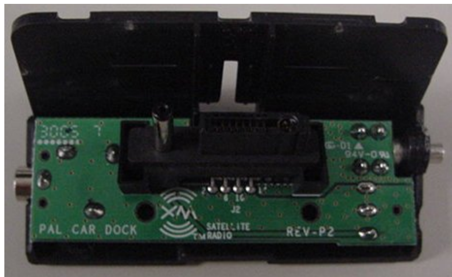
Case Open with PCB Inside
