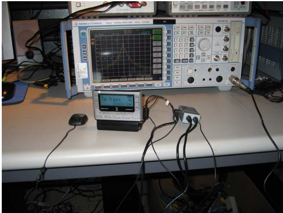
Occupied Bandwidth, Test Setup
