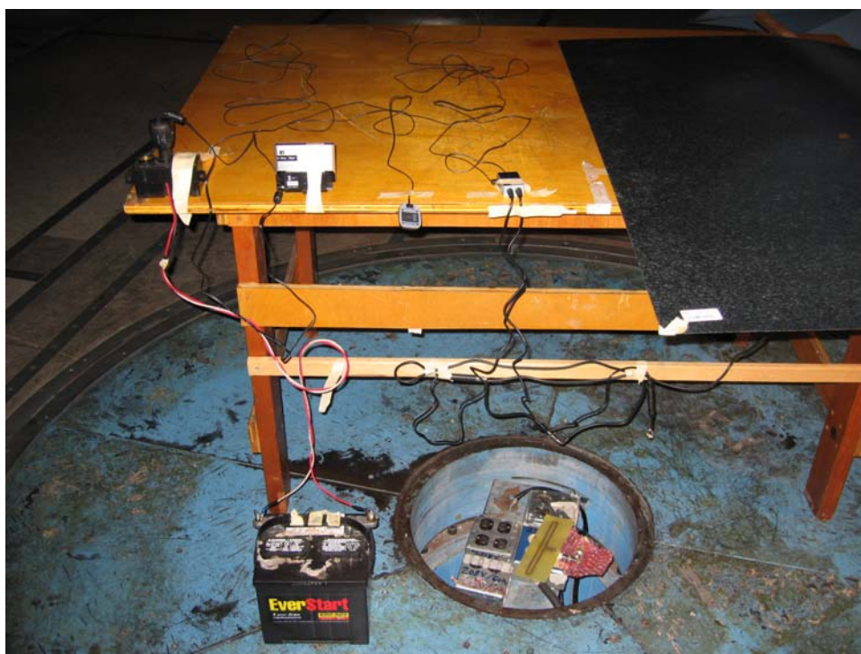
RadyXT with FM Direct, View 2
