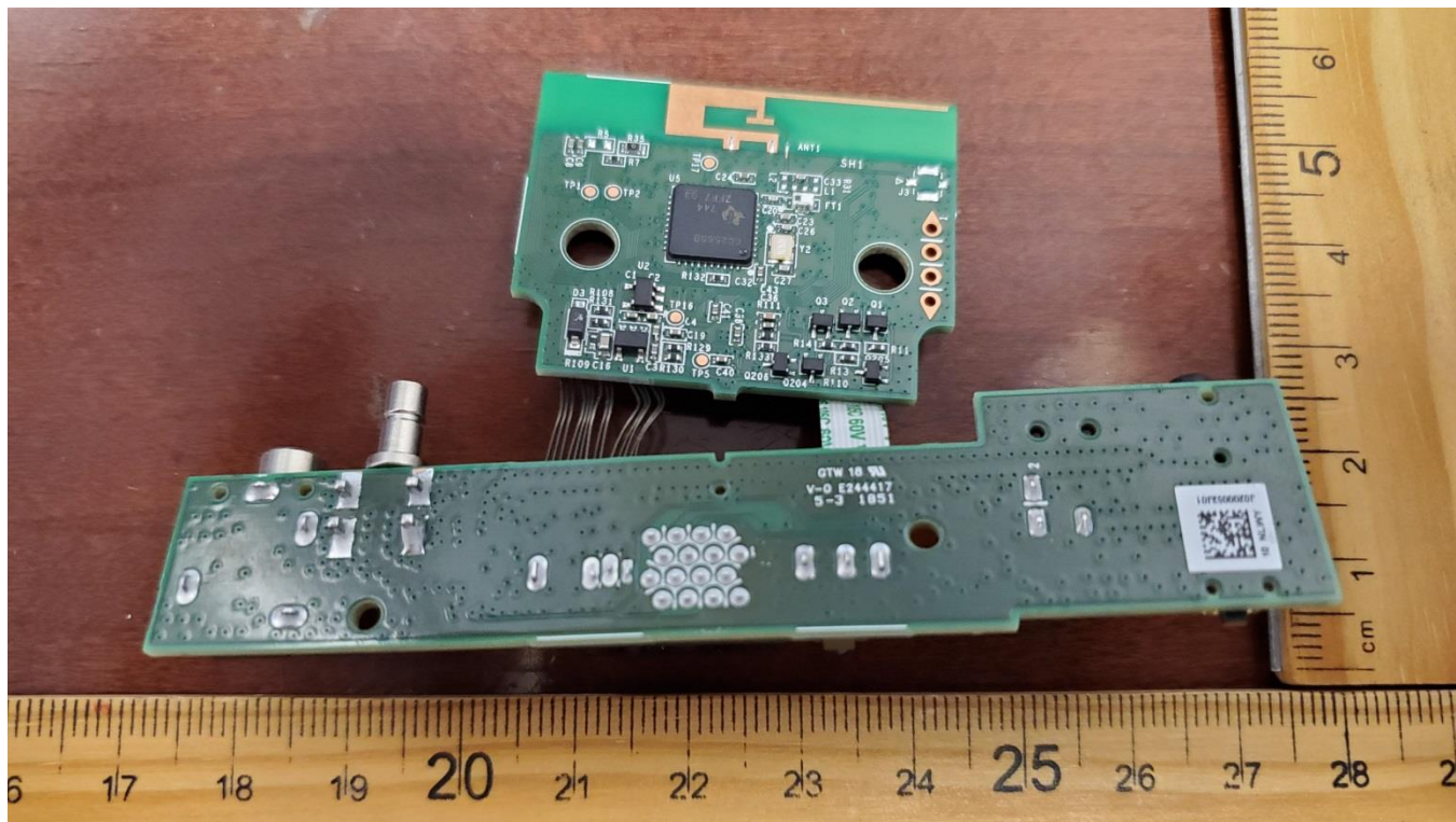
Figure 2: Bottom Side
