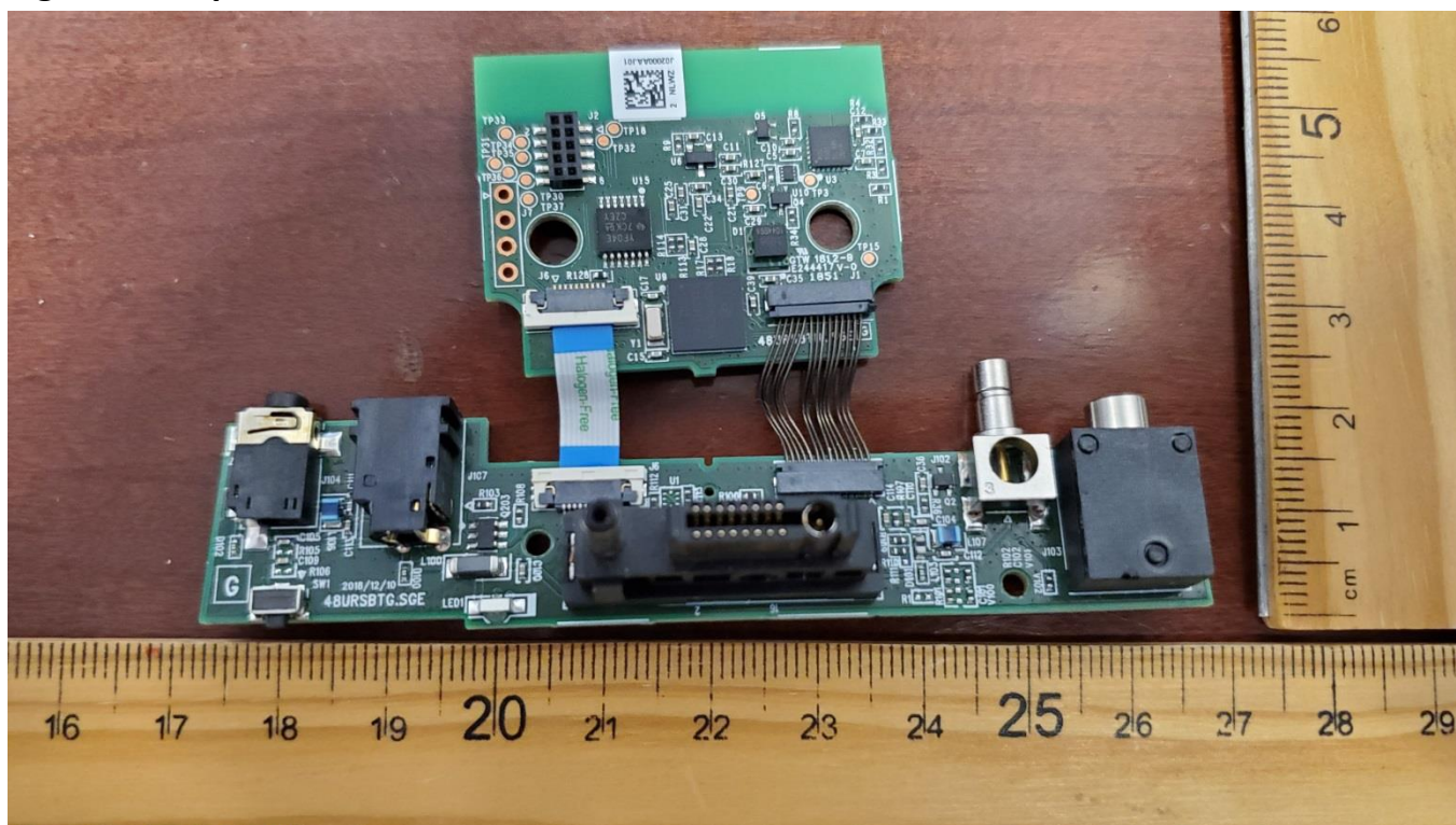
Figure 1: Top side
