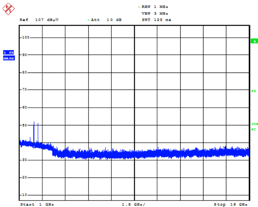
Plot 7-3. Radiated Spurious Plot above 1GHz (Configuration #2, Pol. H)
