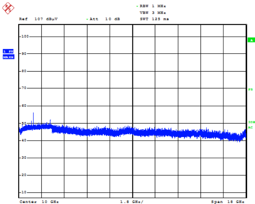
Plot 7-11. Radiated Spurious Plot above 1GHz (Configuration #4, Pol. H)
