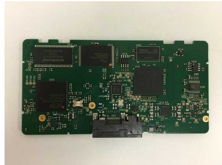
PCBA Rear View (no housing or screws)
