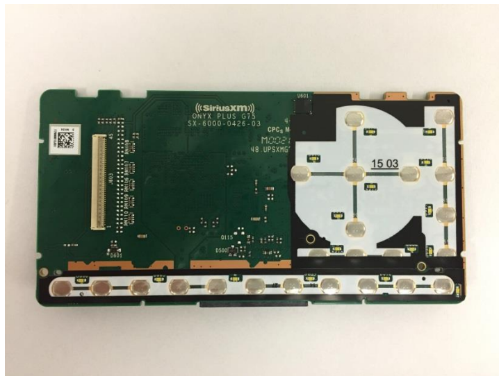
PCBA Front View (w/popple domes)
