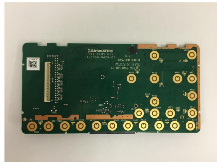
PCBA Front View (no popple domes)
