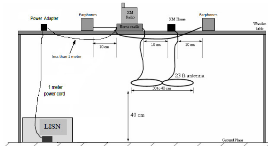
Figure 7-2. Test Instrument & Measurement Setup (Configuration #1)
