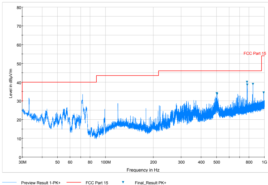
7-6. Radiated Spurious Plot below 1GHz (Configuration #3, Pol. V)
