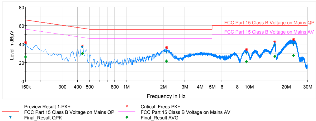
Plot 7-13. Line Conducted Plot (L1, Configuration #1)
