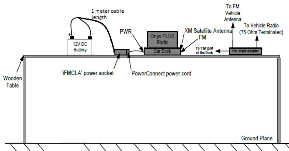
Figure 7-4. Test Instrument & Measurement Setup (Configuration #3)
