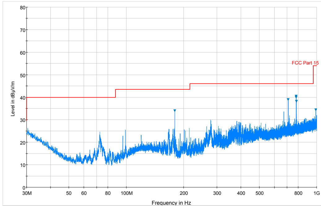
7-9. Radiated Spurious Plot below 1GHz (Configuration #4, Pol. H)
