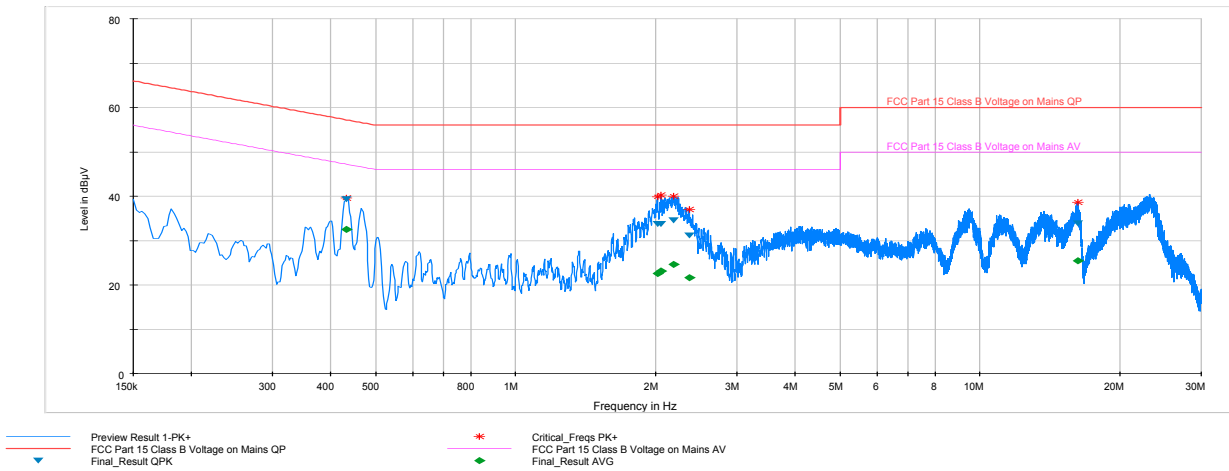
Plot 7-14. Line Conducted Plot (LN, Configuration #1)
