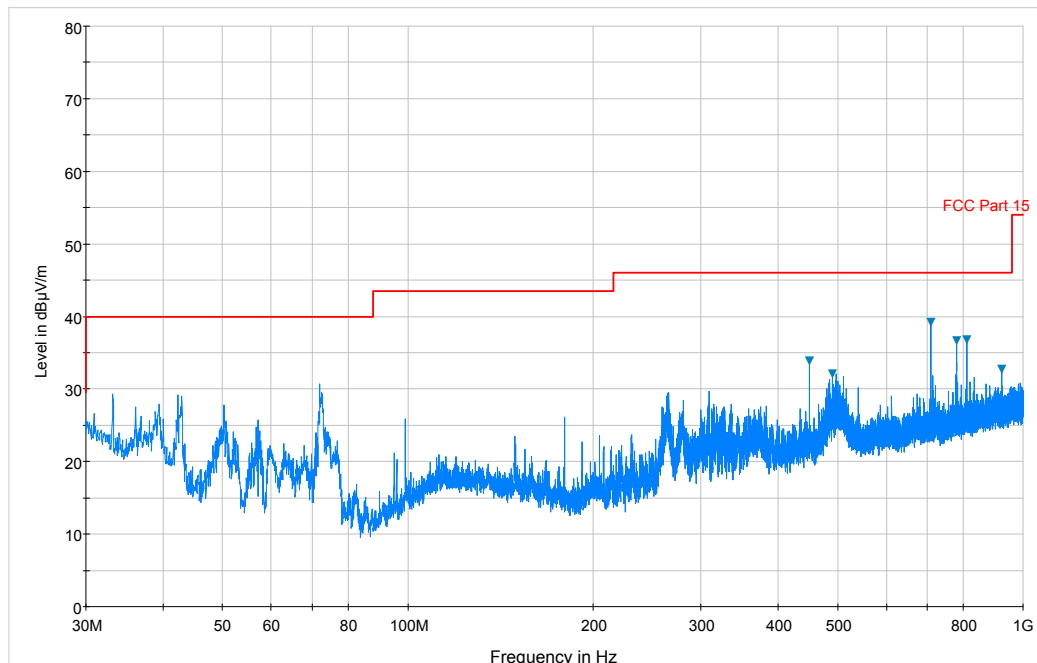
7-10. Radiated Spurious Plot below 1GHz (Configuration #4, Pol. V)
