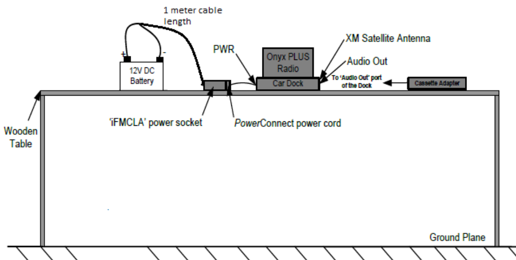
Figure 7-5. Test Instrument & Measurement Setup (Configuration #4)
