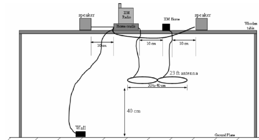
Figure 7-3. Test Instrument & Measurement Setup (Configuration #2)
