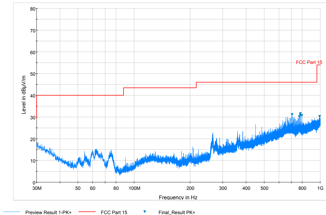
7-2. Radiated Spurious Plot below 1GHz (Configuration #2, Pol. V)
