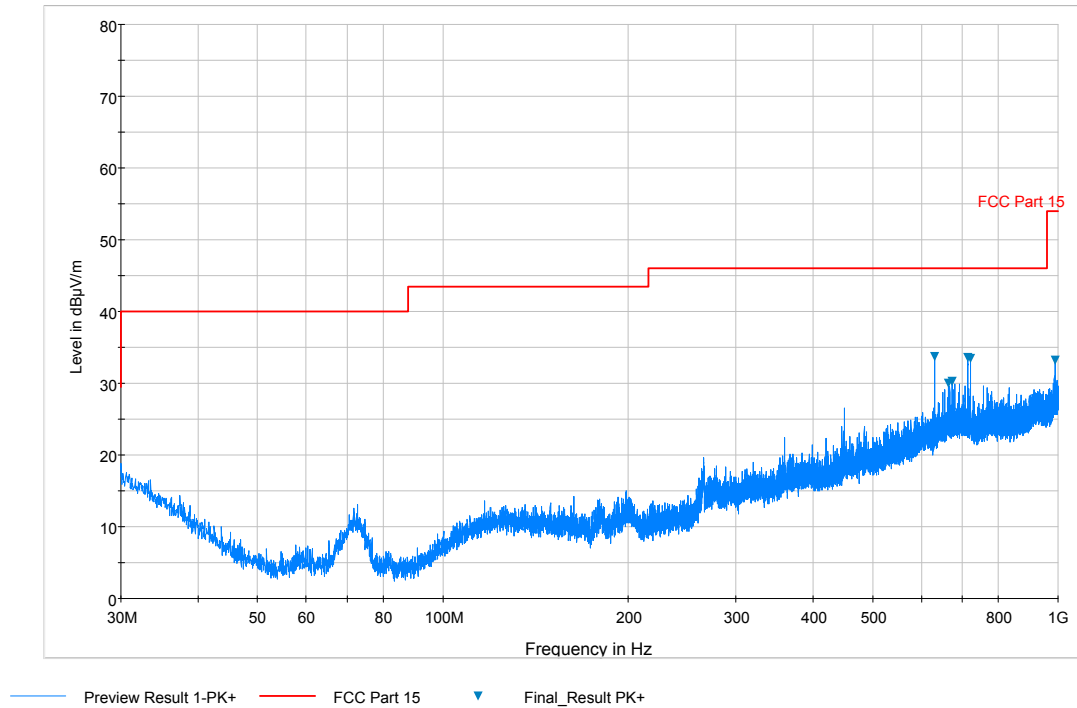
7-1. Radiated Spurious Plot below 1GHz (Configuration #2, Pol. H)
