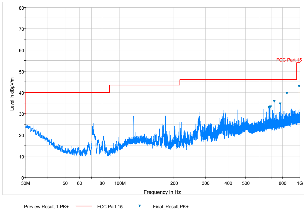
7-5. Radiated Spurious Plot below 1GHz (Configuration #3, Pol. H)
