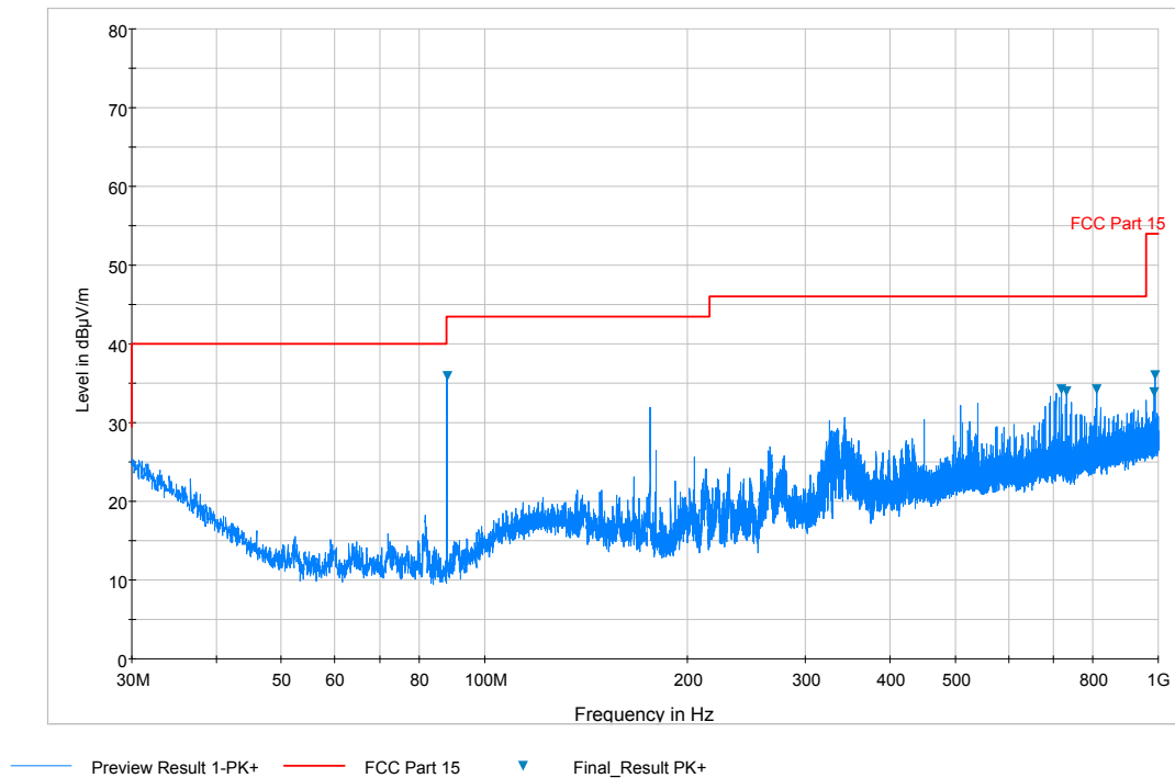
Plot 6-13. Radiated Spurious Plot below 1GHz (Pol. H, Low Channel – 88.1MHz)
