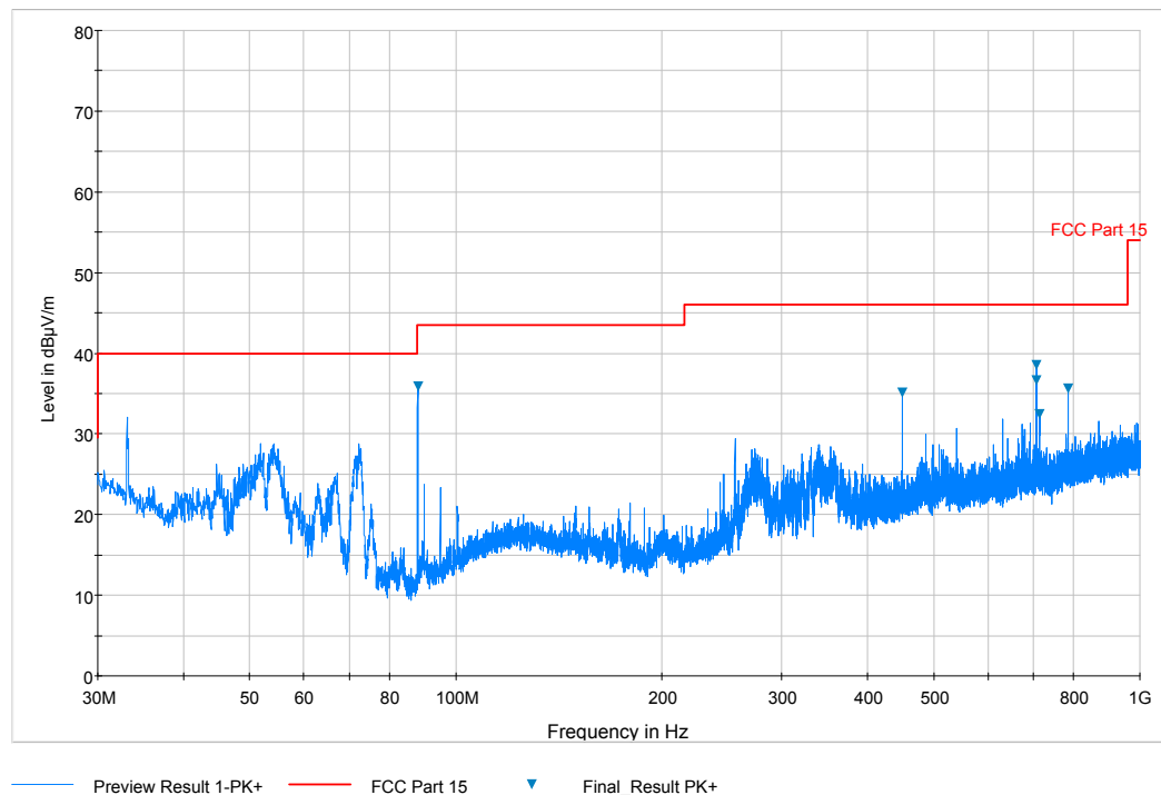
Plot 6-8. Radiated Spurious Plot below 1GHz (Pol. V, Low Channel – 88.1MHz)
