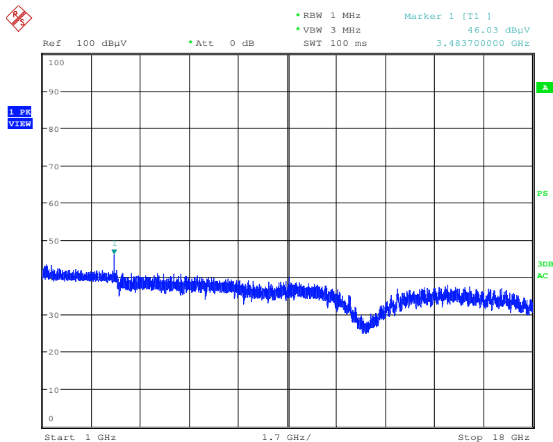
Plot 6-27. Radiated Spurious Plot above 1GHz (Ant. Pol. H, Mid Channel – 96.9MHz)
