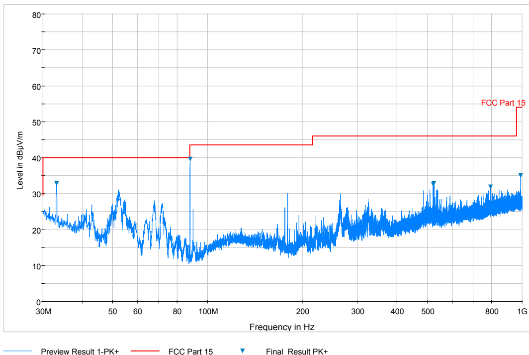
Plot 6-14. Radiated Spurious Plot below 1GHz (Pol. V, Low Channel – 88.1MHz)
