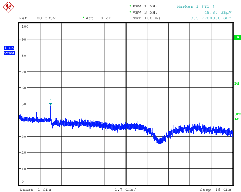
Plot 6-25. Radiated Spurious Plot above 1GHz (Ant. Pol. H, Low Channel – 88.1MHz)
