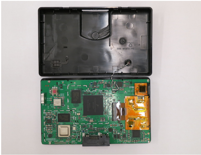
PCBA Rear View (w/back housing removed) PCBA Rear View (w/front housing & screws)
