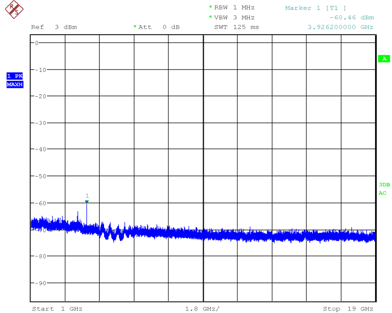
Plot 8-32. Radiated Spurious Plot above 1GHz (Ant. Pol. H, High Channel – 107.9MHz)
