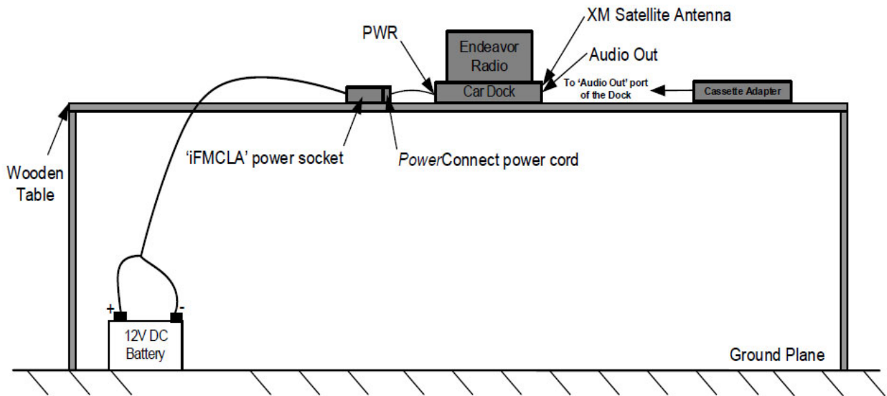
Figure 7-3. Test Instrument & Measurements setup (Configuration #4)
