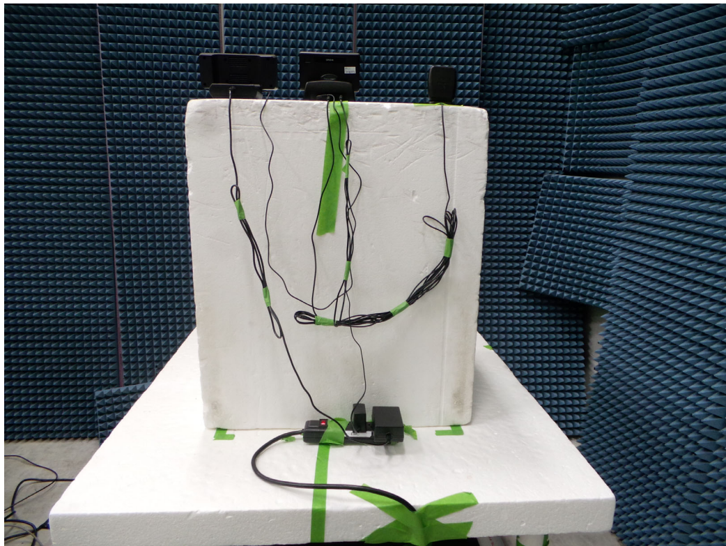
Test Configuration 12: Endeavor with Home Dock (rear)
