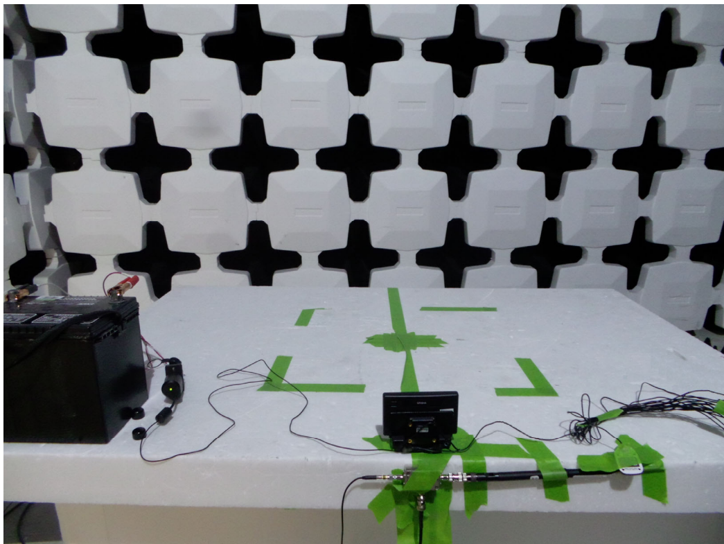
Test Configuration 8 / 11: Endeavor with Vehicle Dock and PowerConnect (rear)
