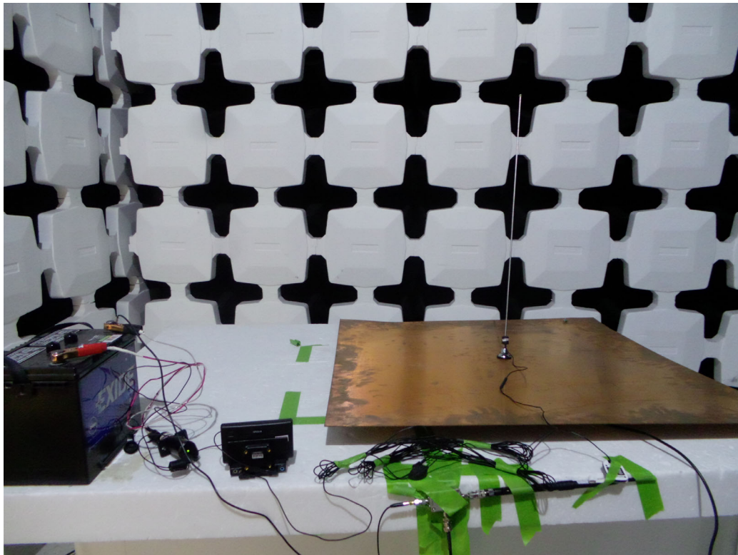
Test Configuration 9: Endeavor with Xpress Car Dock and SureConnect Adapter (rear)
