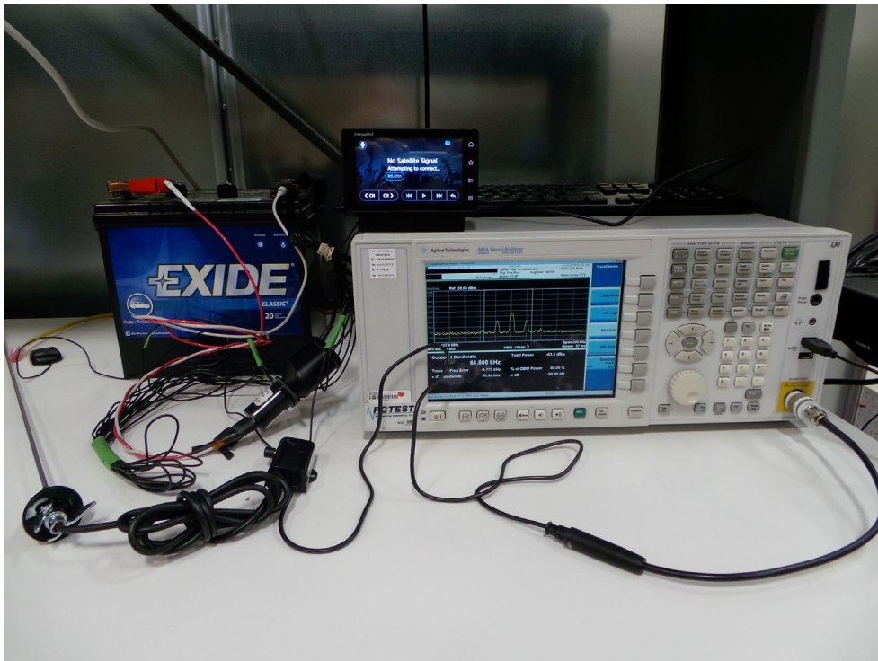
Test Configuration 6: Endeavor with Xpress Car Dock and FM Adapter
