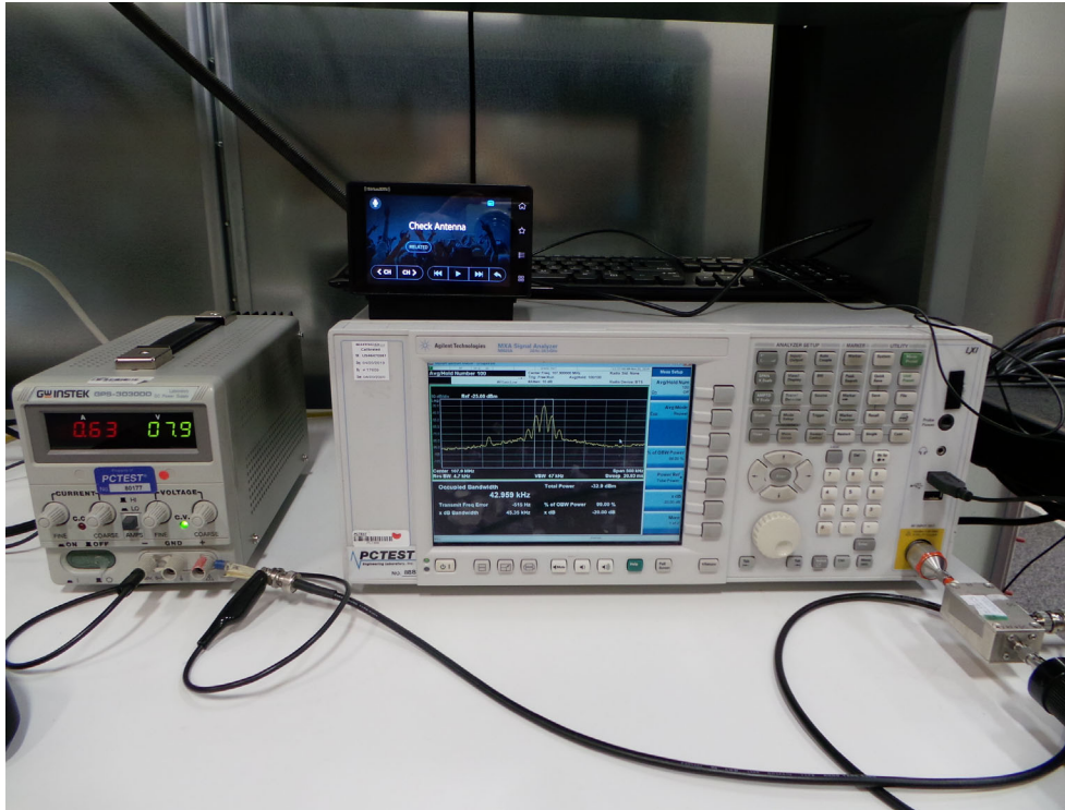
Test Configuration 5 / 10: Endeavor with PowerConnect Car Dock
