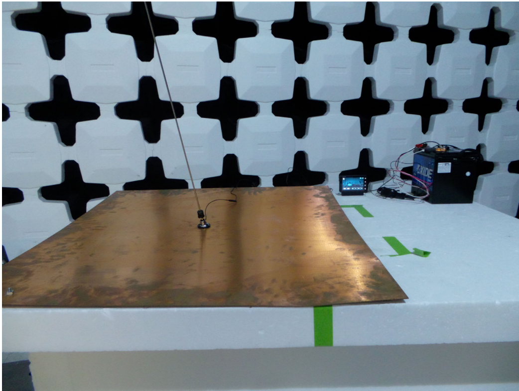
Test Configuration 9: Endeavor with Xpress Car Dock and SureConnect Adapter (front)
