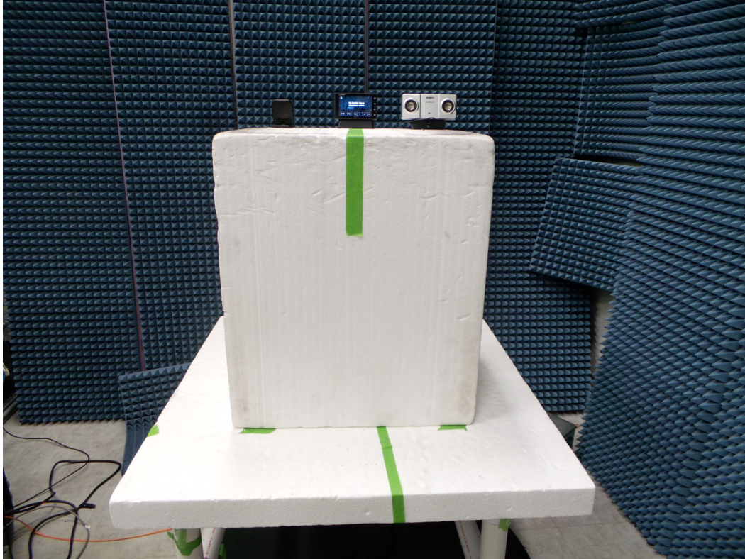
Test Configuration 12: Endeavor with Home Dock (front)
