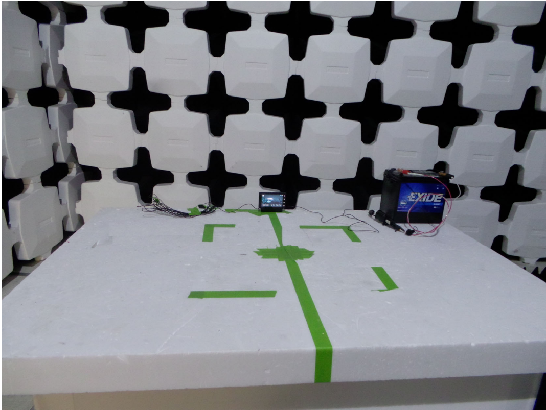
Test Configuration 8 / 11: Endeavor with Vehicle Dock and PowerConnect (front)
