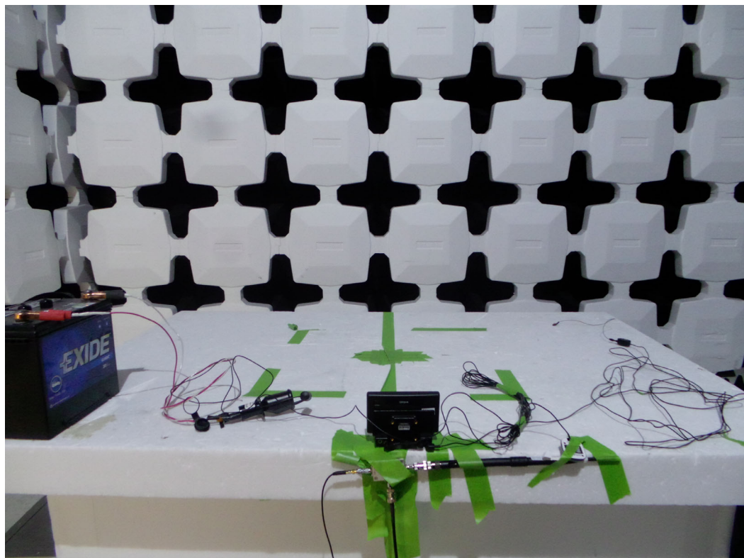
Test Configuration 7: Endeavor and FEA unit (rear)
