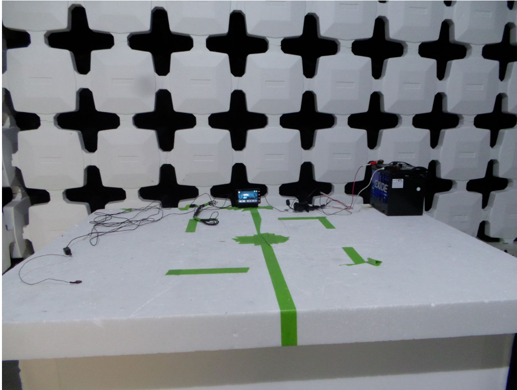
Test Configuration 7: Endeavor and FEA unit (front)
