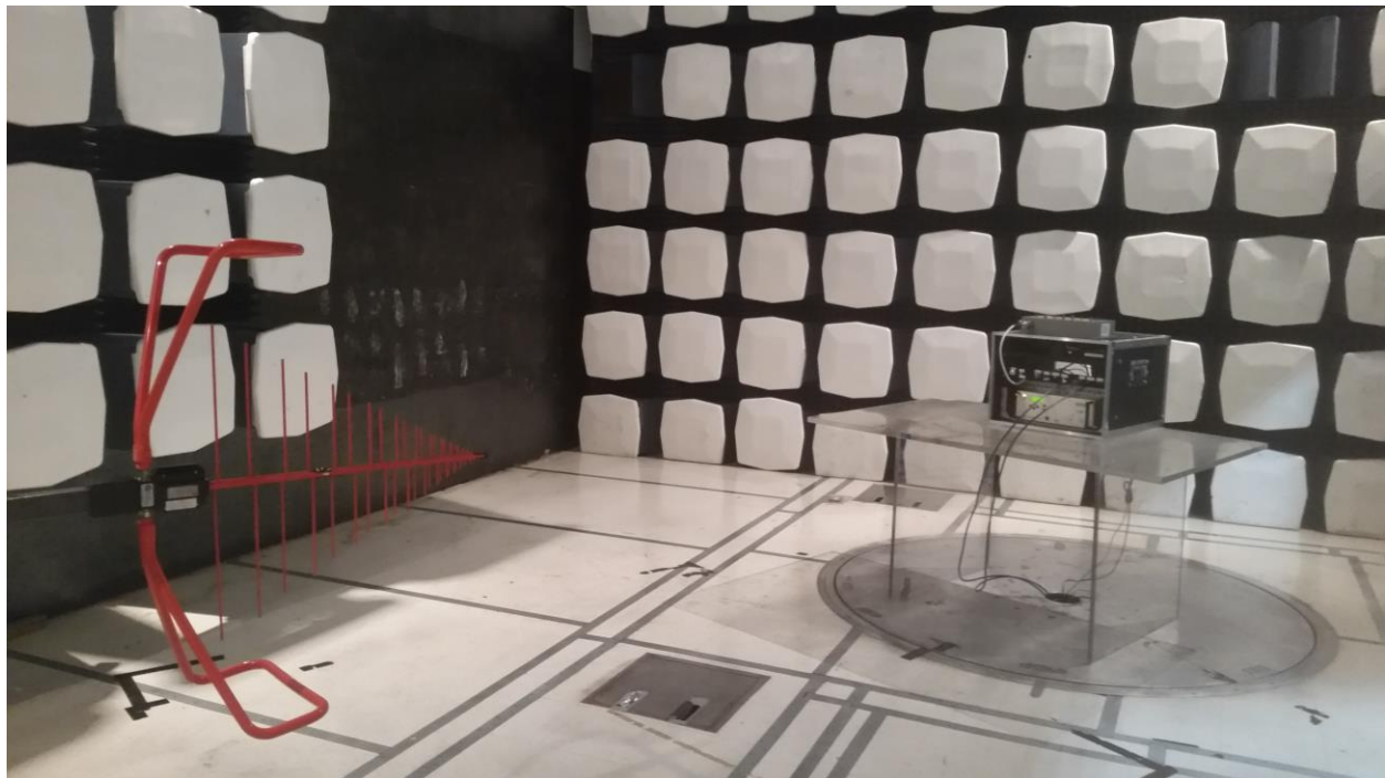
Photograph 4. Radiated Emissions, Below 1 GHz
