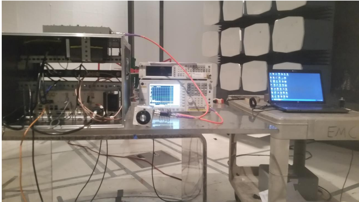
Photograph 1. Conducted Measurement Setup
