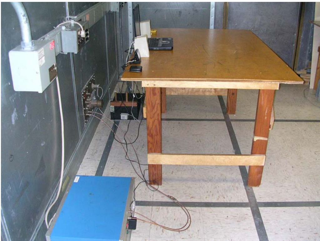
Photo 4 : Conducted Emissions – EUT in Home Cradle – side view
