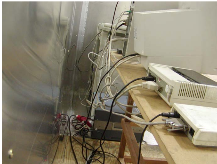
Conducted Emission Setup – Side View
