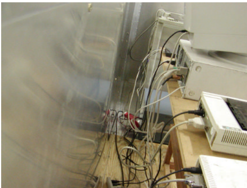
Conducted Emission Setup – Side View
