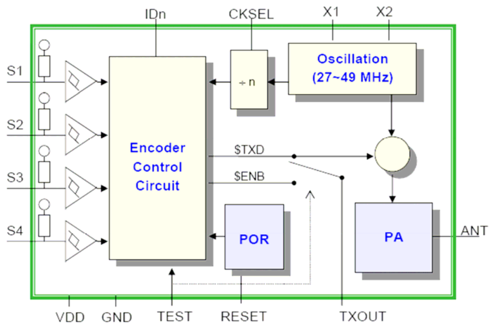
W55RFS27T1B System Block Diagram
