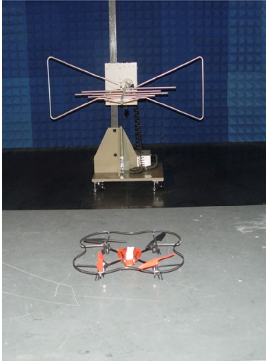
Radiated emissions test 30MHz- 1GHz
