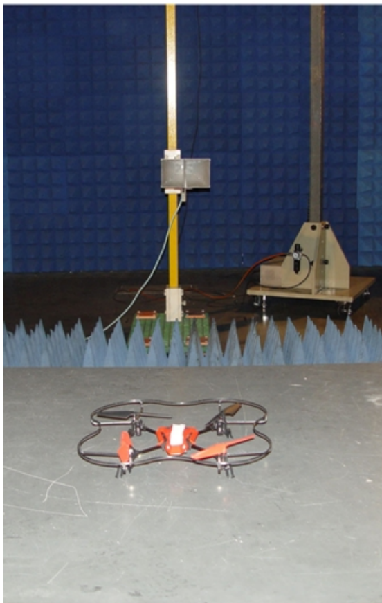
Radiated emissions test > 1GHz
