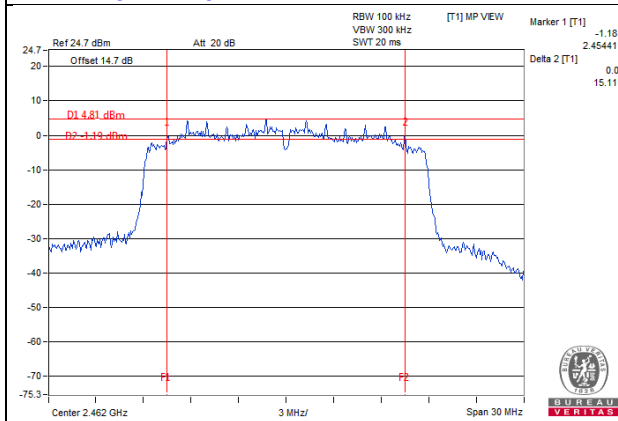
802.11n (20MHz) 2Tx CDD mode Chain1 CH11
